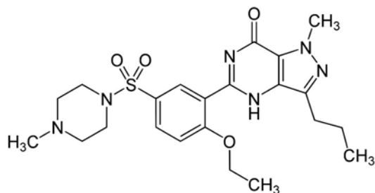
Fig. 1 Molecular structure of sildenafil
