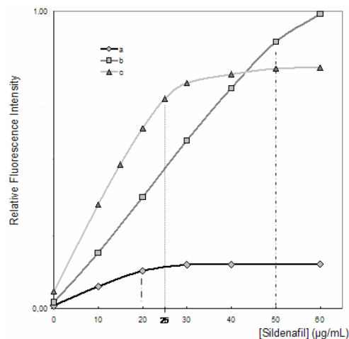
Fig. 7 Calibration curve of sildenafil in absence and presence of surfactants
