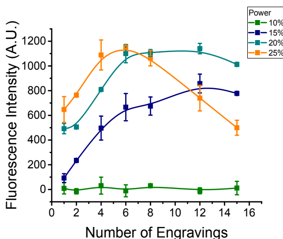
Figure 3b: Effect of the number of engraving steps on the fluorescence intensity. Experiments performed using 95% speed.
