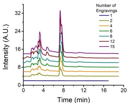
Figure 5: HPLC-FD analysis of the compounds formed by laser engraving (varying the number of engravings at 20% power and 95% speed) and extracted in H 2 O.
