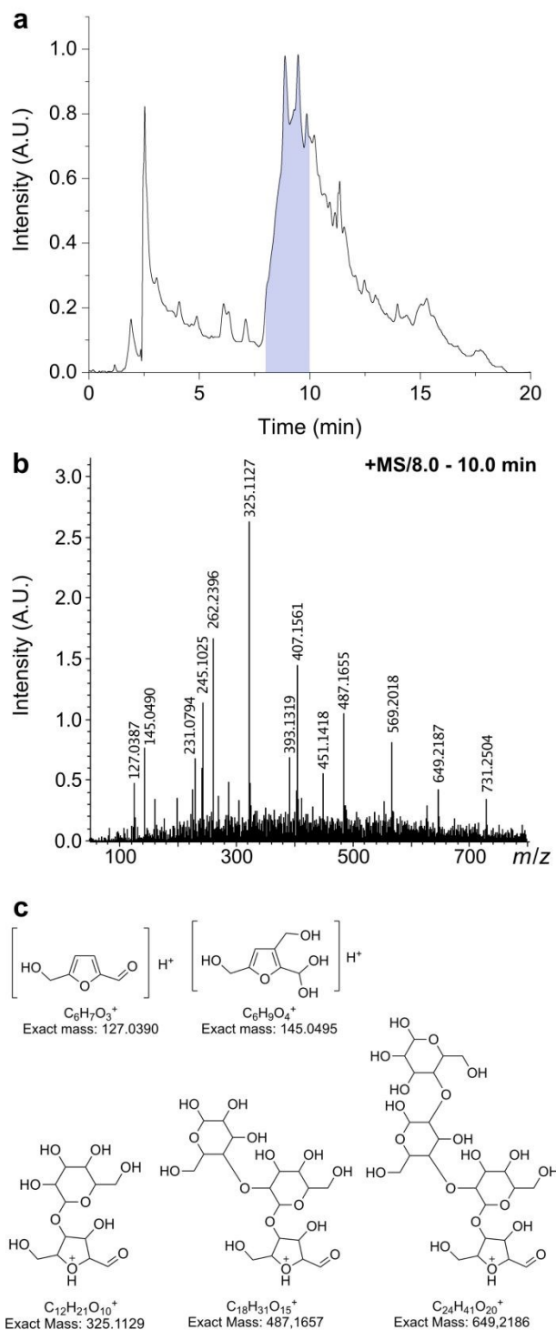
Figure 6: Characterization of the fluorescent species in engraved paper by HPLC-HRMS-PDA-FD. (a) Chromatogram obtained with fluorescence detection ( \lambda_{\text{EX}} = 370 \text{ nm} / \lambda_{\text{EM}} = 450 \text{ nm} ). The blue filling indicates the region of higher fluorescence intensity. (b) Mass spectra of the species with retention time ranging from 8 to 10 min. (c) Chemical structures of species with exact mass compatible with the experimental m/z .
