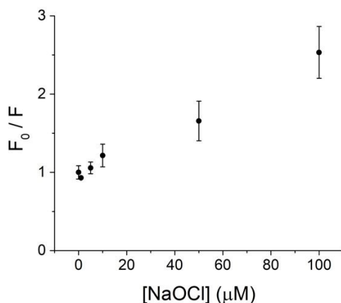
Figure 7a: Dependence of the fluorescence quenching with respect to the concentration of sodium hypochlorite. Paper was treated with 20% power, 95% speed for 15 engravings. 4 μL of hypochlorite solutions were added to the rastered spots of paper. Fluorimeter Excitation: 365 nm, Emission: 440 nm (n=4)
