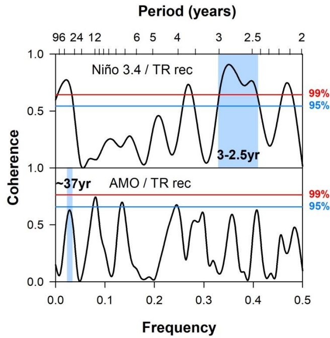
Figure 4. Cross-spectral coherence computed between the precipitation tree-ring reconstruction (TR rec) and Niño 3.4 SST (above) and AMO index (below). Horizontal lines indicate the 99 and 95% confidence intervals. Precipitation reconstruction and Niño 3.4 SST are in phase and highly coherent at a period between 2.5 to 3 years (above 99% also indicated by shading), while the precipitation reconstruction and AMO index are in phase at a period of ~ 37 years (approaching 95%, indicated by shading).
