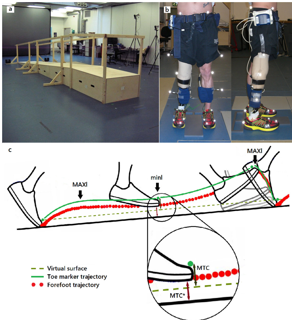
Fig. 1. Data collection protocol. a) Set up of the ramp (modular design). The inclined walk way was 6 m long, 1 m wide and 5° inclination. It was custom made and incorporated a raised surface at its upper end to provide a stable area for resting and turning. b) Marker set used in the study. c) Estimation of the walking surface and MTC. MTC*: MTC according to definition, MTC: the value of MTC calculated in this study, MAXI: local maximum and mini: local minimum.
