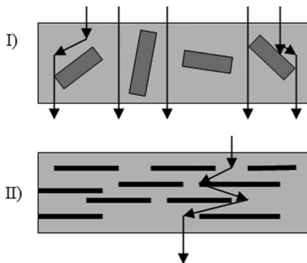
Figure 11 Tortuous diffusion path of conventional composites (I) and polymer/clay nanocomposites (II).
