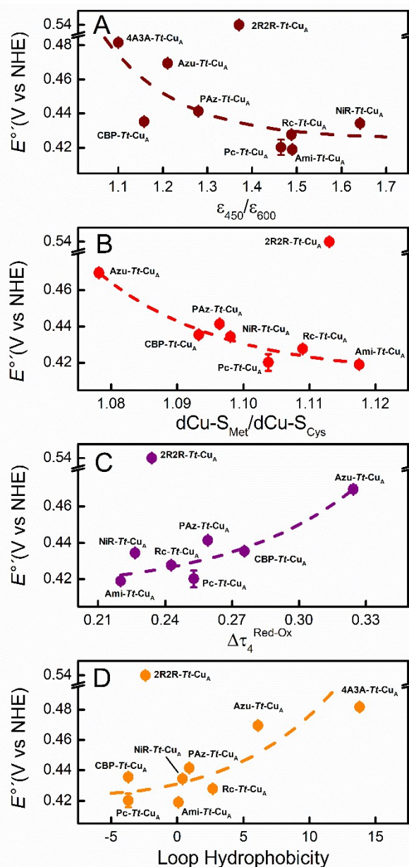
Figure 5. Reduction potentials of the Tt -Cu A chimeras as function of (A) the experimental \epsilon_{450}/\epsilon_{600} ratio, (B) the calculated dCu-S Met /dCu-S Cys ratio, (C) the calculated \Delta\tau_4 = \tau_4(\text{red}) - \tau_4(\text{ox}) parameter and (D) the hydrophobicity of the ligand loop. Dashed curves are included to guide the eye. Error bars represent the standard deviation of no less than 3 independent measures.
