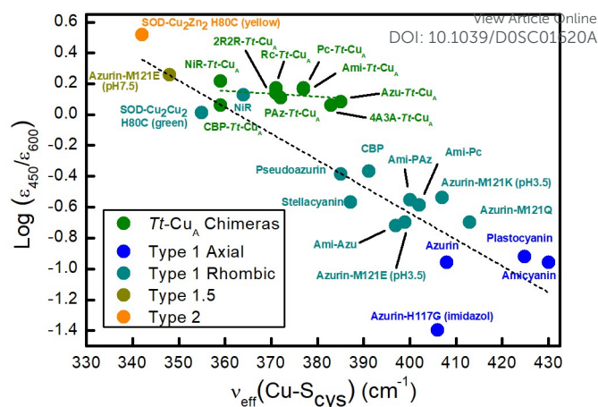
Figure 3. Correlation of the \epsilon_{450}/\epsilon_{600} ratio with the Cu-S Cys effective stretching frequency for different types of mono-copper sites. Green symbols correspond to the Tt-Cu A chimeras from this work. The rest of the symbols are data taken from literature 5,52,55 for different types of mononuclear Cu centers, as indicated in the inset, and include axial and rhombic T1 centers, one T2 site and one so-called T1.5 center of geometry intermediate between T1 and T2 sites. 52 Dashed lines are included to guide the eye.
