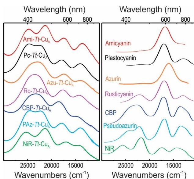
Figure 2. Left: Electronic absorption spectra of the chimeras engineered in the Tt -Cu A scaffold. Right: Electronic absorption spectra of wild type proteins that harbor T1 copper sites taken from literature. 40,41,44–47 Spectra of the 2R2R- Tt -Cu A and 4A3A- Tt -Cu A variants, as well as spectral deconvolutions, are shown in Figure S1.
