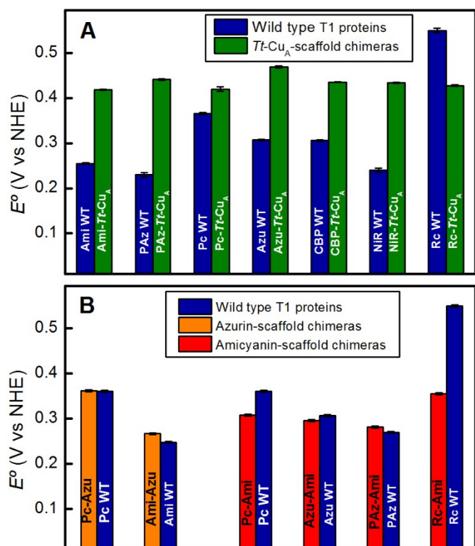
Figure 4. (A) Reduction potentials of the Tt -Cu A chimeras compared with the corresponding native T1 sites. (B) Reduction potentials of chimeras based on the azurin and amicyanin scaffolds compared to the corresponding native sites. Except for Tt -Cu A chimeras, values are taken from literature. 5,13,45
