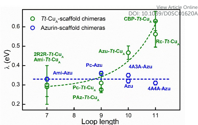
Figure 6. Reorganization energies of Tt-Cu A -based chimeras (green; this work) and azurin-based chimeras (blue; taken from Monari et. al. 85 ) as a function of the length of the ligand loop. Dashed curves are included to guide the eye. Error bars represent the standard deviation of no less than 3 independent measures.
