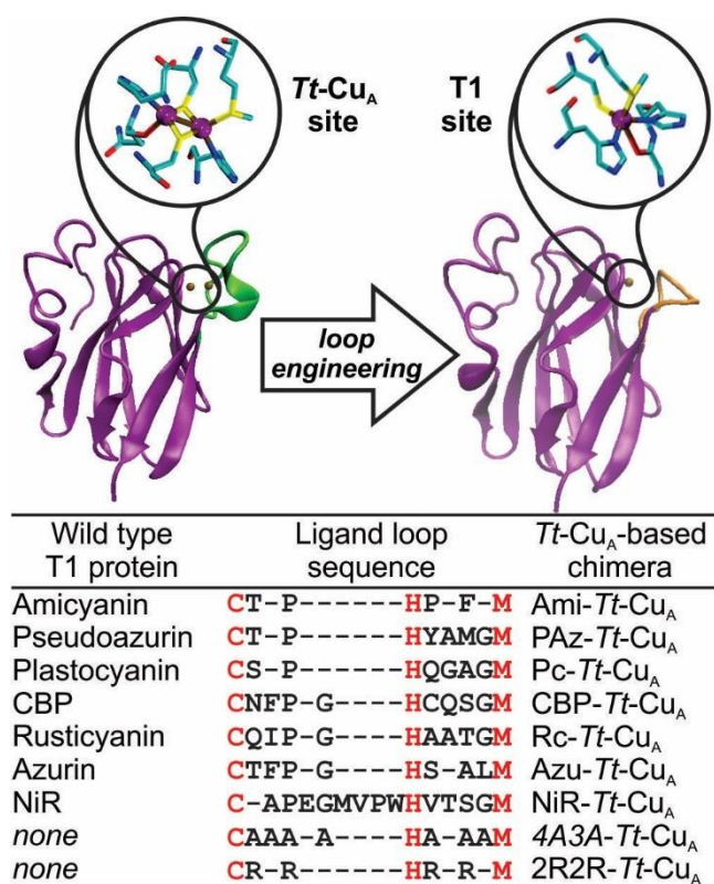
Figure 1. X-ray crystallographic structures of native Tt -Cu A (left; PDB ID 2CUA) 38 on the left, and that of Ami- Tt -Cu A on the right (right; PDB ID 5U7N). 36 The loop replaced in the chimeras is indicated in green and orange, respectively. The loop sequences employed to obtain the different chimeras are listed below. Red letters denote the conserved ligand set.
