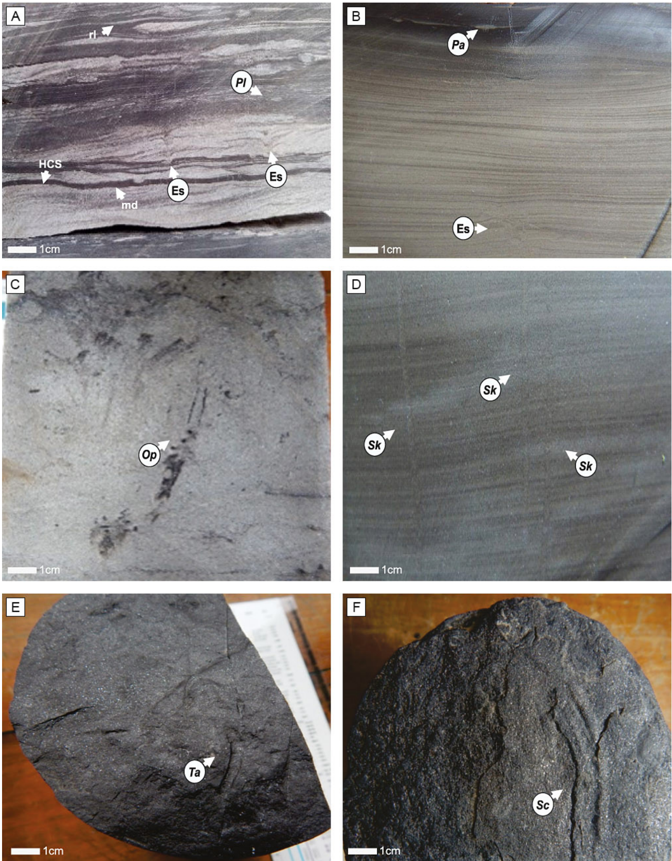
Figure 5. Core photographs showing the sedimentary structures and traces fossils of F3 and F4 facies defined in the Los Monos Formation. a) Facies 3, Ramos x-12 borehole, 2714.5 mbgs; ripples cross lamination (rl), micro hummocky cross lamination (HCS), mud drapes (md), escape trace fossils (Es) and Planolites (Pl). b) Facies 4, Aguas Blancas xp-13 borehole, 2813.5 mbgs; Palaeophycus (Pa). c) Ophiomorpha (Op). d) Skolithos (Sk). e) Taenidium (Ta). f) Scolicia (Sc).
