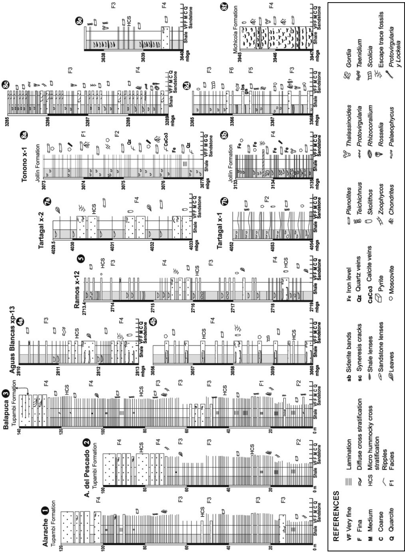
Figure 3. Sedimentary logs of the Los Monos Formation. Logs ubication in Fig. 1.
