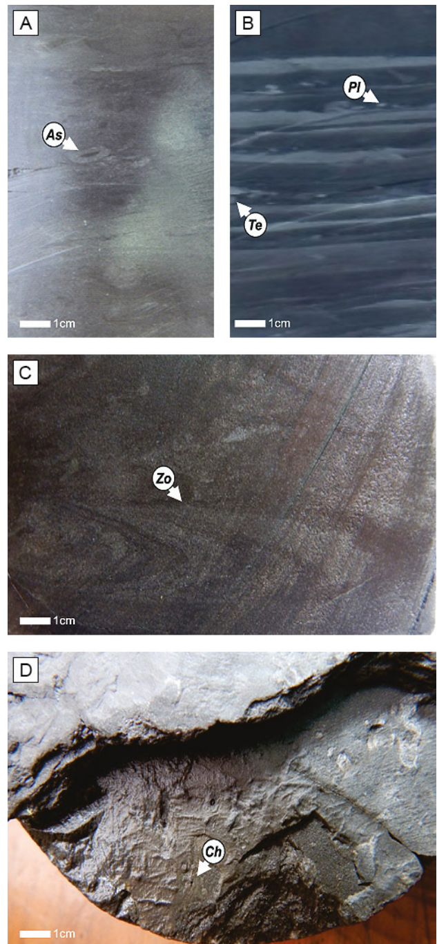
Figure 4. Core photographs showing the sedimentary structures and trace fossils of F1 and F2 facies defined in the Los Monos Formation. a) Facies 1, Aguas Blancas xp-13 borehole, 2810.5 mbgs; Asterosoma (As). b) Facies 2, Aguas Blancas xp-13 borehole, 2811 mbgs; Planolites (Pl), Teichichnus (Te). c) Zoophycos (Zo). d) Chondrites (Ch).
