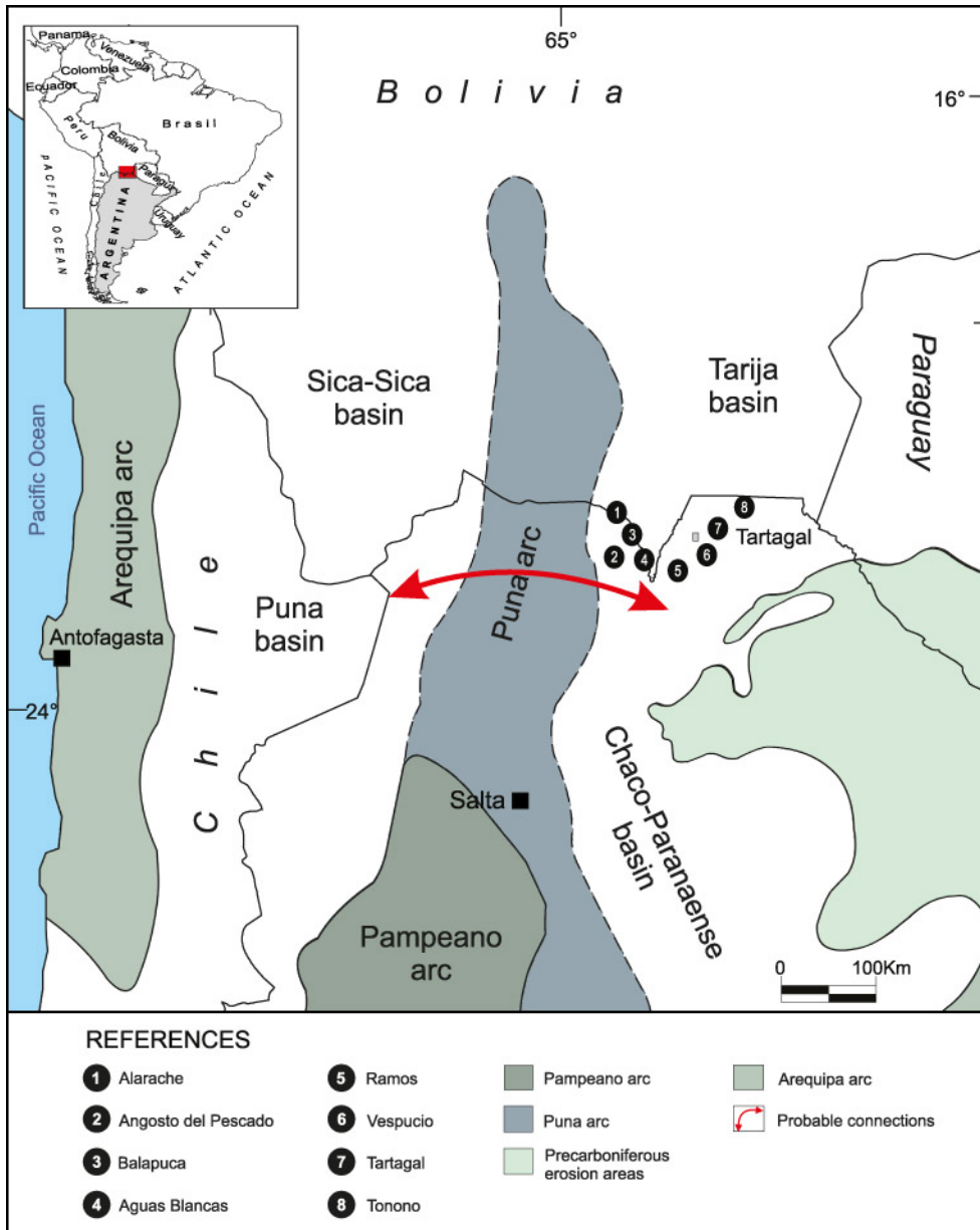
Figure 1. Location of study localities within the Tarija Basin.
