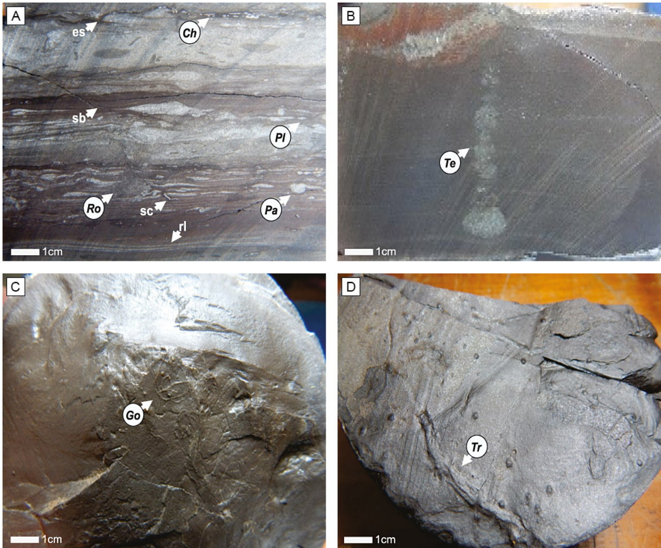
Figure 6. Core photographs showing the sedimentary structures and traces fossils of F5 defined in the Los Monos Formation. a) Facies 5, Tonono x-1 borehole, 3366.5 mbgs, to the top transgressive lag; Planolites (Pl), Rosselia (Ro) and Palaeophycus (Pa) with siderite bands (sb) and syneresis cracks (sc), ripples cross lamination (rl) and erosive surface to the top (es). b) Teichichnus (Te). c) Gordia (Go). d) Treptichnus (Tr).
