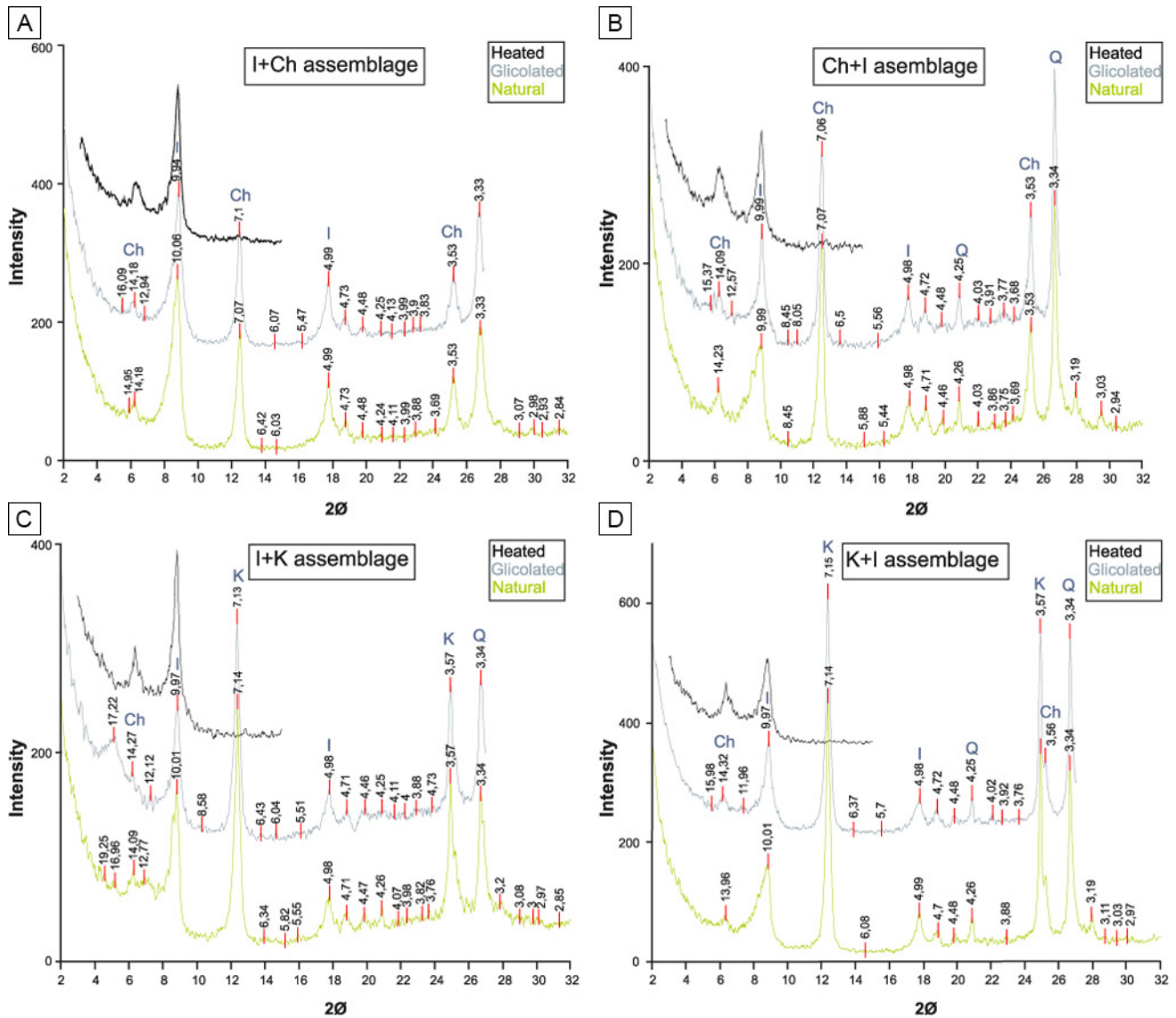
Figure 7. X-ray diffractograms of the clay assemblages from Los Monos Formation. a) Illite+Chlorite assemblage (I+Ch). b) Chlorite+Illite assemblage (Ch+I). c) Illite+Kaolinite assemblage (I+K). d) Kaolinite+Illite assemblage (K+I).
