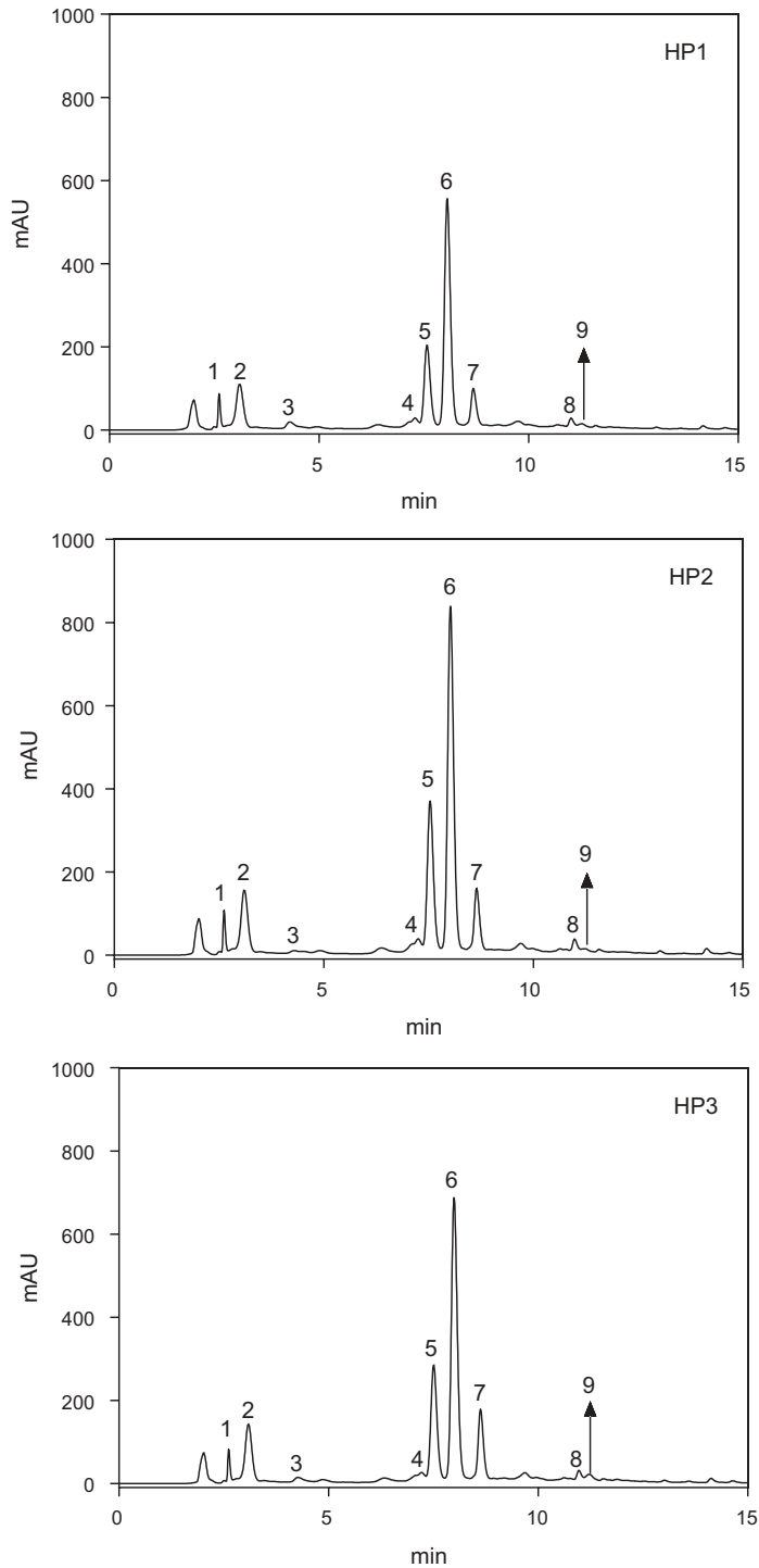
Figure 2. HPLC chromatograms of different phenolic compounds in SPL at 326 nm for different harvest period. Peaks 1 is 5- O -caffeoylquinic acid; peak 2 is 3- O -caffeoylquinic acid; peak 3 is caffeic acid; peak 4 is isoquercetin; peak 5 is 3,4-di- O -caffeoylquinic acid; peak 6 is 3,5-di- O -caffeoylquinic acid; peak 7 is 4,5-di- O -caffeoylquinic acid; peak 8 is 3,4,5-tri- O -caffeoylquinic acid; peak 9 is quercetin.
