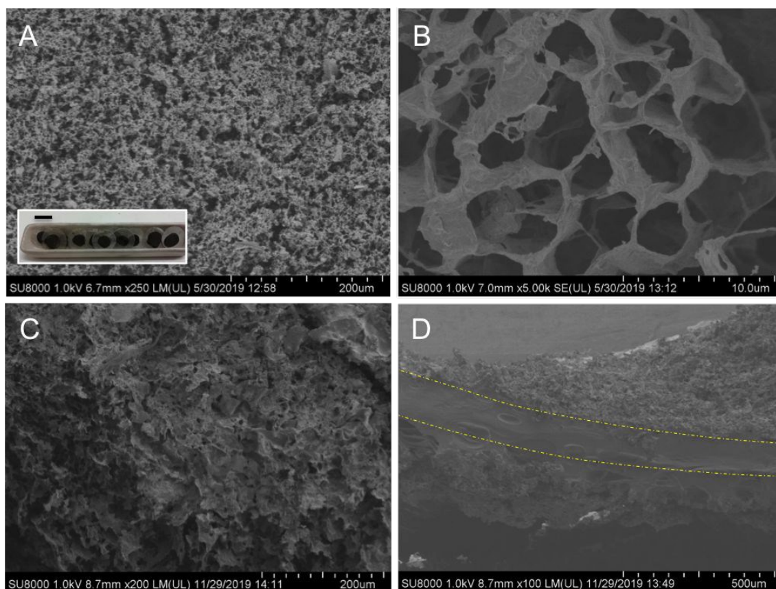
Figure 5. SEM characterization of the macroporous graphene electrode material. (A-B) SEM images corresponding to the graphene before the gel infiltration. (C) Surface of the graphene after infiltration with the biohydrogel electrolyte. (D) Cross-section of the Graphene/biohydrogel/Graphene electrochemical cell. The dash-dot lines in the figure are guide for the eye. Inset Figure 5A: Graphene electrodes supported on stainless steel mesh. Length of the scale bar: 11 mm.
