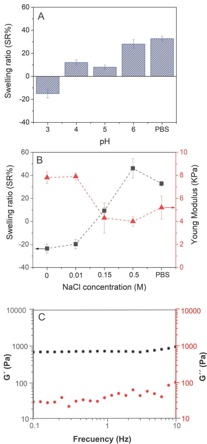
Figure 4. (A) Swelling ratio of ChS-gel hydrogels as a function of pH (NaCl=0.15 M). (B) Swelling ratio and Young's modulus of ChS-gel hydrogels as a function of NaCl concentration (pH=4) and (C) Oscillatory frequency sweeps corresponding to a ChS-gelatin hydrogels swollen in PBS.
