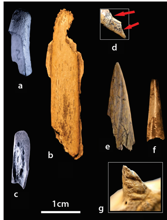
Fig. 4. Different tool-types referred to in the text: a antler tine tentatively identified as a flaker (BP2-2); b smoother made from a macromammal rib (BP2-8); c hide scraper (BP2-48); d Cathartidae cf. Cathartes-Coragyps distal radius splinter (BP2-70) with arrows showing the mastic residues; e pin-like tool (BP2-20); f pin-like tool (BP2-19); g awl (BP2-54).
