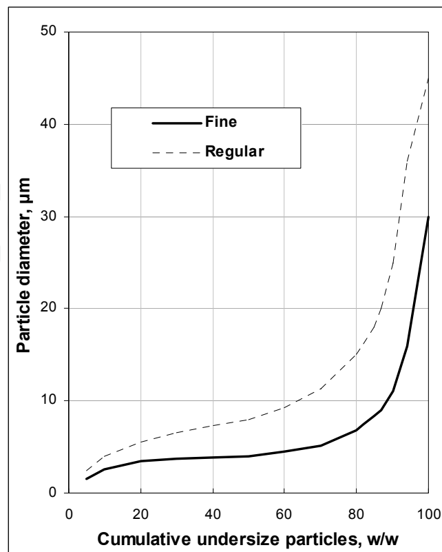
Fig. 1. Commercial spherical zinc dusts. D 50/50 average particle diameters: 4 \mu\text{m} (fine) and 8 \mu\text{m} (regular).
