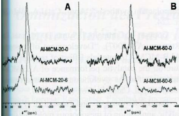
Figura 2: RMN de: (A) Al-MCM-20-0 y Al-MCM-20-6. (B) Al-MCM-60-0 y Al-MCM-60-6.
