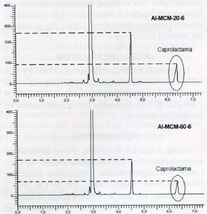
Figura 3: Cromatogramas: Al-MCM-20-6 y Al-MCM-60-6.
