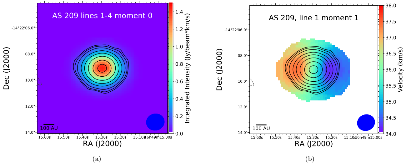
Figure 1. Integrated intensity (moment 0) map for hyperfine components 1-4 (a), and velocity (moment 1) map for hyperfine 1 (b). The moment maps are created from line emission with intensity \geq 5\sigma_{Iline} . Contours represent total intensity (Stokes I ) of 3, 10, 50, 100, 200, 325 and 500\sigma levels.
