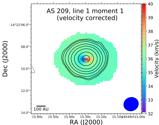
Figure 2. Velocity (moment 1) map for hyperfine 1, made using data corrected for Keplerian rotation using gofish . Contours represent total intensity (Stokes I ) of 3, 10, 50, 100, 200, 325 and 500\sigma levels.
