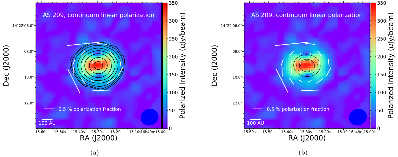
Figure 5. 1.3 mm continuum linear polarization in AS 209. The black contours in (a) represent total intensity (Stokes I ) of 3, 10, 50, 100, 200, 325 and 500\sigma levels. The solid contours in (b) represent the locations of rings, and the dashed contours represent the locations of gaps from (Fedele et al. 2018). The colormap represents debiased polarized intensity with the scale on the right of each source. The length of the polarization vectors corresponds to the polarization fraction. The vectors are plotted with \sim 5 segments per beam. Vectors are only plotted where the polarized intensity P \geq 3\sigma_P and P/I \geq 0.1 .
