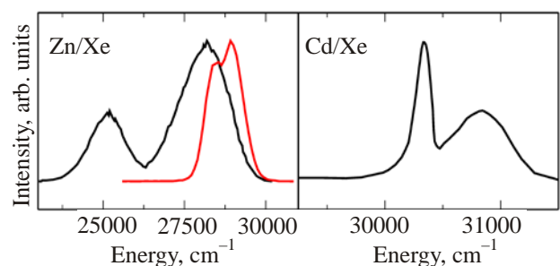
Fig. 8. Experimental (black) and calculated (red) emission bands associated to ^3P_1-^1S_0 photoexcitation of Zn atoms trapped in Xe matrices (left). Experimental emission bands associated to ^1P_1-^1S_0 photoexcitation of Cd atoms trapped in Xe matrices (right).
