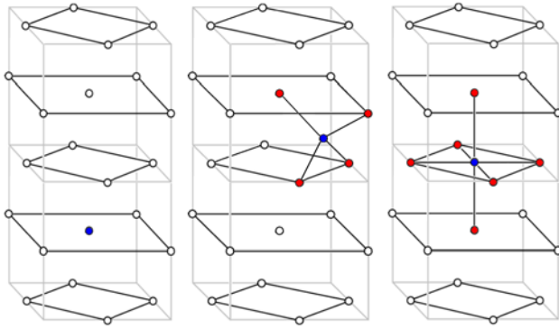
Fig. 2. (Color online) Models of the three vacancy sites considered in this work. Shown from left to right are the single vacancy sv , tetra-vacancy tv and hexa-vacancy hv sites. The empty circles represent RG atoms in the fcc lattice, the blue circles show the position of the guest M atom in each model while the red circles indicate the locations of the removed RG atoms forming the specific vacancy. The octahedral vacancy ( ov ) site mentioned in Fig. 1 is not shown. It corresponds to the removal of 12 RG atoms surrounding the guest metal atom. In this diagram it would correspond to the removal of all the RG atoms surrounding the metal atom in the bottom of the structure shown in left panel of the figure.
