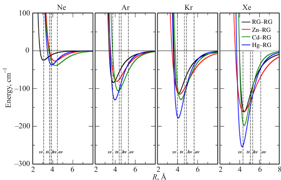
Fig. 1. (Color online) Comparison of the ground state interatomic M( ^1S_0 )–RG (colored coded traces) and RG–RG (black traces) pair-potentials. The broken vertical lines represent interatomic distances of the sv , tv , hv and ov (octahedral) vacancy sites in the solid rare gases Ne, Ar, Kr and Xe.
