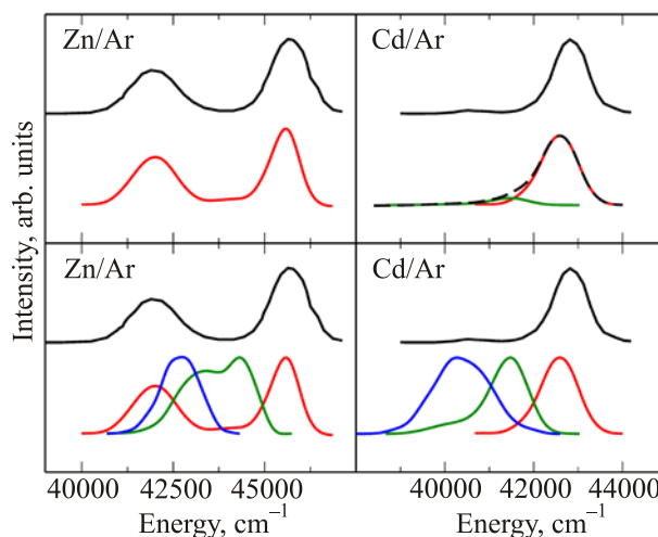
Fig. 6. (Color online) The emission spectra of ^1P_1-^1S_0 transition of Zn (left) and Cd (right) atoms trapped in Ar matrices. In all panels on top are presented experimental spectra for annealed samples, and on bottom are shown the contributions of sv (red), tv (green) and hv (blue) sites obtained from MDQT simulations. Top panels show the calculated weighted contributions for each site. The black dashed line corresponds to the weighted sum of all site contributions.
