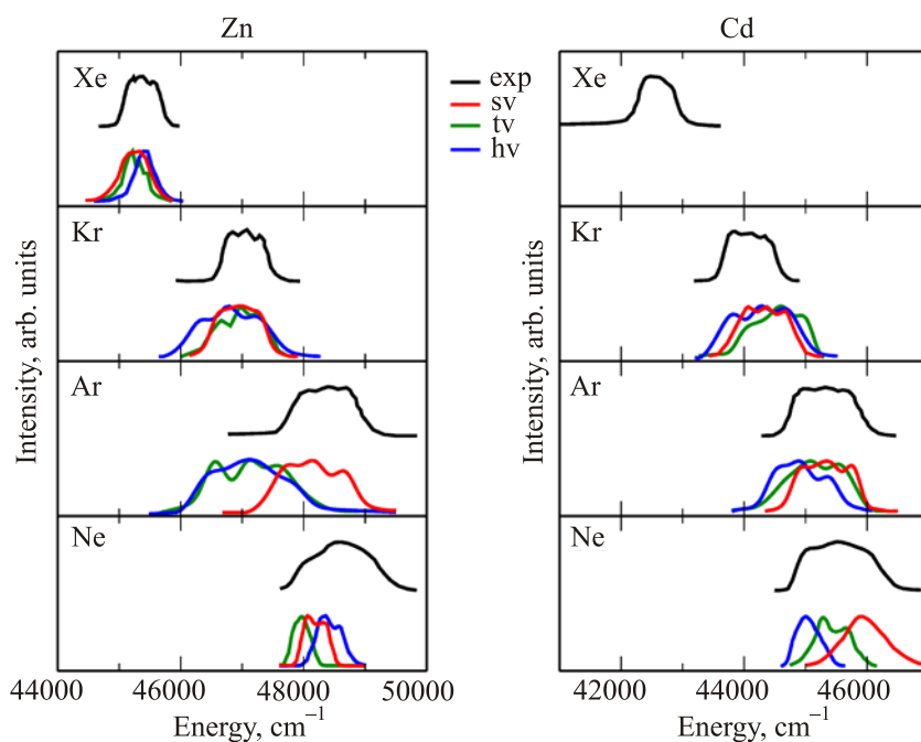
Fig. 3. (Color online) Absorption bands arising from the ^1P_1 \leftarrow ^1S_0 transition that takes place for the metal atoms Zn and Cd trapped in four rare gas matrices Ne, Ar, Kr and Xe. On the top of each panel, the experimental bands are represented with black solid lines. The simulated absorption bandshapes of the three sites are shown colour coded — red for sv , green for tv and blue for hv sites.
