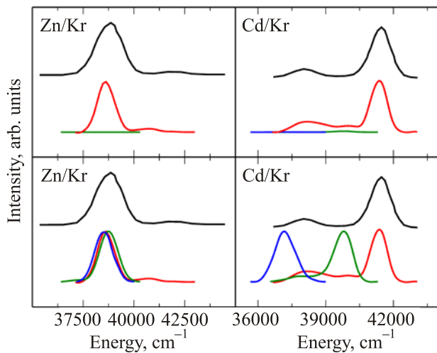
Fig. 7. (Color online) Simulated emission spectra for the ^1P_1-^1S_0 transition of Zn (left) and Cd (right) atoms trapped in Kr matrices. In all panels on top are presented experimental spectra for annealed samples, and on bottom are shown the contributions of sv (red), tv (green) and hv (blue) sites obtained from MDQT simulations. Top panels show the calculated weighted contributions for each site.
