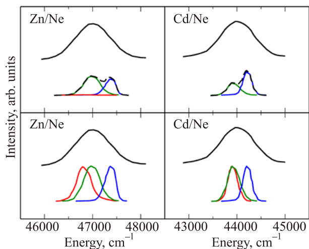
Fig. 5. (Color online) The emission spectra of ^1P_1-^1S_0 transition of Zn (left) and Cd (right) atoms trapped in Ne matrices. In both panels the experimental spectra are presented on the top by the black traces. On the bottom the contributions of sv (red), tv (green) and hv (blue) sites obtained from MDQT simulations are shown colour coded. The top panels show the calculated weighted contributions for each site as specified in Table 3. The black dashed line corresponds to the weighted sum of all site contributions.
