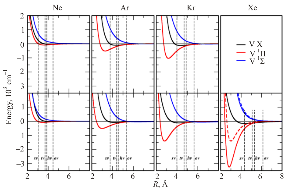
Fig. 4. (Color online) Interatomic potential curves X, ^1\Pi and ^1\Sigma for molecular complex 1:1 M-RG. Top panels for Cd/RG and bottom panels for Zn/RG.
