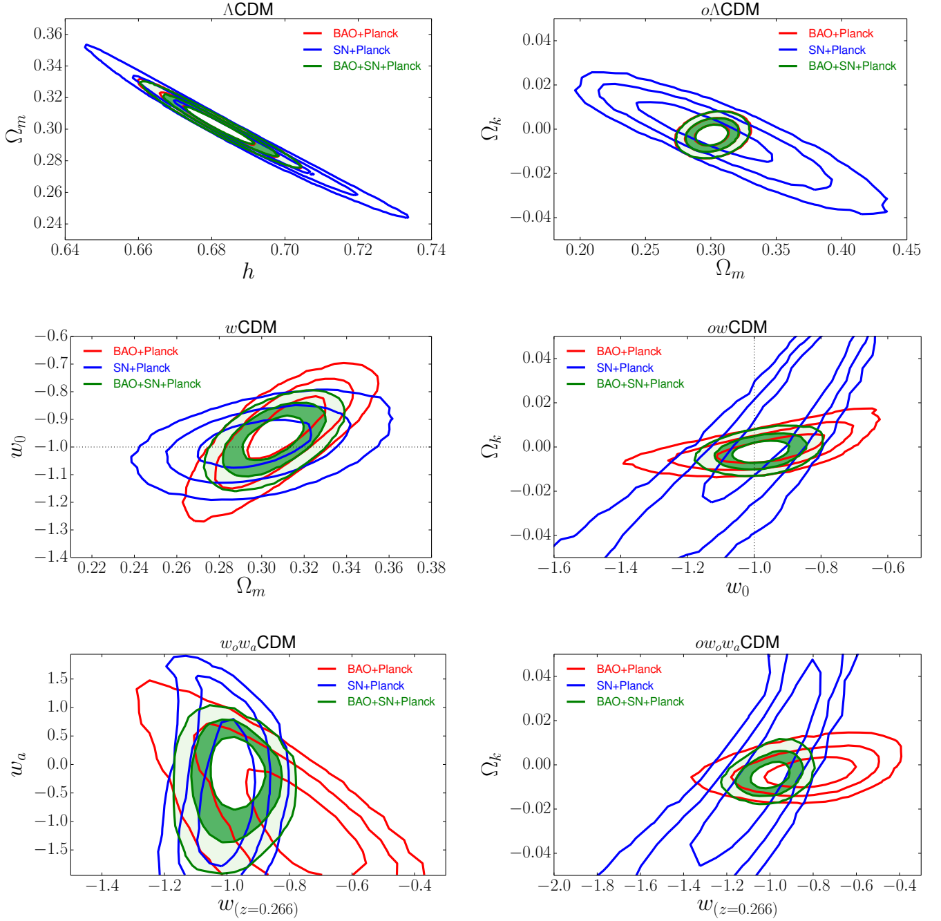
Figure 8. Constraints on interesting parameter combinations in a variety of dark energy models: \Lambda CDM (upper left), o\Lambda CDM (upper right), w CDM (middle left), ow CDM (middle right), w_0w_a CDM (bottom left) and ow_0w_a CDM (bottom right). Curves show 68%, 95%, and 99.7% confidence contours for the data combinations indicated in the legend. In the top panels the red contours are almost fully obscured by the green contours because the BAO+Planck combination is already as constraining as the BAO+SN+Planck combination, but for models with freedom in dark energy the SN and BAO constraints are complementary. The bottom panels, with evolving w(z) , display the value of w at z = 0.266 , the "pivot" redshift where w is best constrained by BAO+SN+Planck in the w_0w_a CDM model. For our BAO+SN+Planck contours, the white zone interior to the dark green annulus marks the 68% confidence region, and the outer edge of the dark annulus is 95%.
