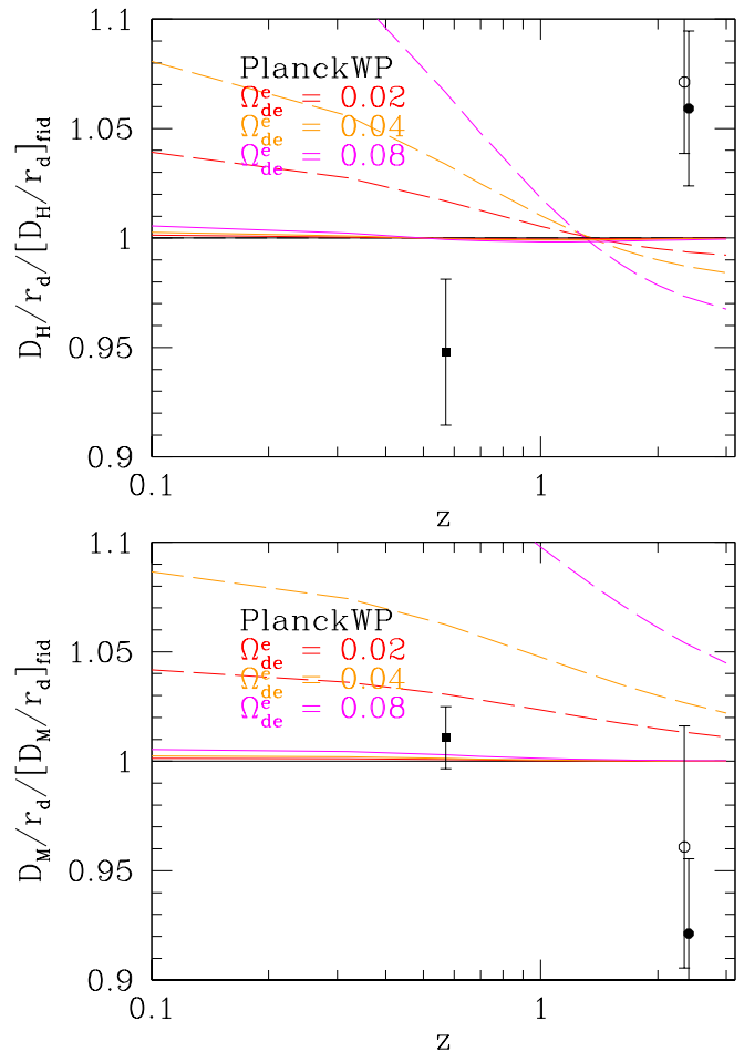
Figure 12. Predicted BAO scales for early dark energy models with CMB observables \Omega_b h^2 , \Omega_m h^2 , and D_M(1090)/r_d held fixed to the values of the best-fit Planck+WP \Lambda CDM model. We adopt equation (25) with w_0 = -1 . Solid lines show the case in which r_d is rescaled by (1 - \Omega_{\text{de}}^e)^{1/2} to represent the effect of early dark energy in the pre-recombination era, while dashed lines show the case in which r_d is held fixed at the fiducial model value of r_d = 147.49 Mpc. We show ratios of D_H(z)/r_d (top) or D_M(z)/r_d (bottom) relative to the fiducial ( \Omega_{\text{de}}^e = 0 ) model. Points with error bars show the BAO measurements from CMASS galaxies at z = 0.57 (filled square) and from Ly \alpha F auto-correlation (open circle) and cross-correlation (filled circle) at z = 2.34 . For visual clarity, the Ly \alpha F cross-correlation points have been slightly shifted in redshift.
