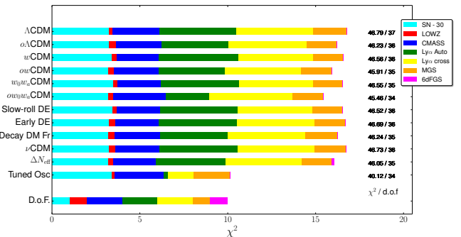
Figure 10. \chi^2 values for the best-fit versions of cosmological models considered in the paper. Each bar represents the minimum \chi^2 for the model listed at the left axis, and colors show the \chi^2 contributions of individual data sets. For better visualization, we subtract 30 from the SN \chi^2 . CMB contributions are not included but (with our 3-parameter compression) are always close to zero. The total \chi^2 and model degrees-of-freedom (d.o.f., 40 data points minus number of fit parameters, which includes the SNIa absolute magnitude normalization as well as cosmological quantities) are listed to the right of each bar. The bottom bar shows the number of d.o.f. associated with each data set. For the \Delta N_{\text{eff}} model we use cosmomc rather than our compressed CMB description, but we again omit CMB contributions to \chi^2 .
