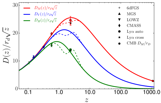
Figure 18. A “tuned oscillation” model in which a Gaussian perturbation of the \Lambda CDM D_M(z) is introduced to allow a good simultaneous fit to the galaxy and Ly \alpha F BAO data. Solid lines show the same \Lambda CDM model plotted in Figure 1, while the dashed line shows the perturbed model.
