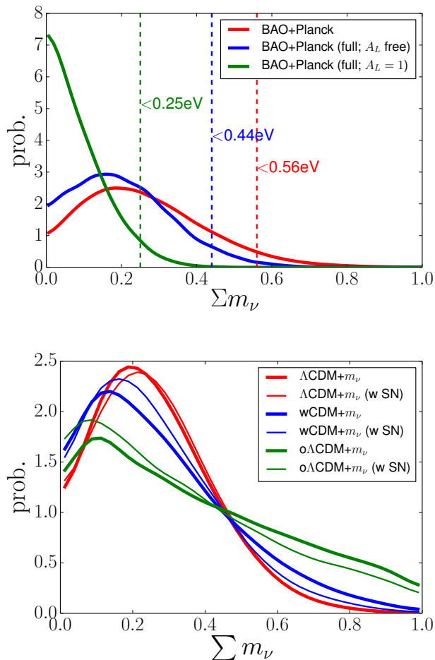
Figure 16. Neutrino mass constraints for several combinations of data and model freedom. In the top panel, the red curve shows the posterior pdf (with a flat prior) on \sum m_\nu from the expansion history constraint on the neutrino mass, based on the combination of BAO with our compressed CMB description, which yields \sum m_\nu < 0.56 eV at 95% confidence. The green curve shows the result obtained by replacing our compressed CMB description with the full Planck+WP power spectrum using cosmomc , which strengthens the upper limit to \sum m_\nu < 0.25 eV. The blue curve adopts the same data combination but additionally marginalizes over the parameter A_L , demonstrating that the difference between the green and red curves is driven mainly by the lensing amplitude information in the Planck data. In the lower panel, curves show the posterior pdf of \sum m_\nu from our usual BAO+Planck (thick) or BAO+SN+Planck (thin) geometrical constraints, assuming \Lambda CDM, w CDM, or o\Lambda CDM (red, blue, green, respectively).
