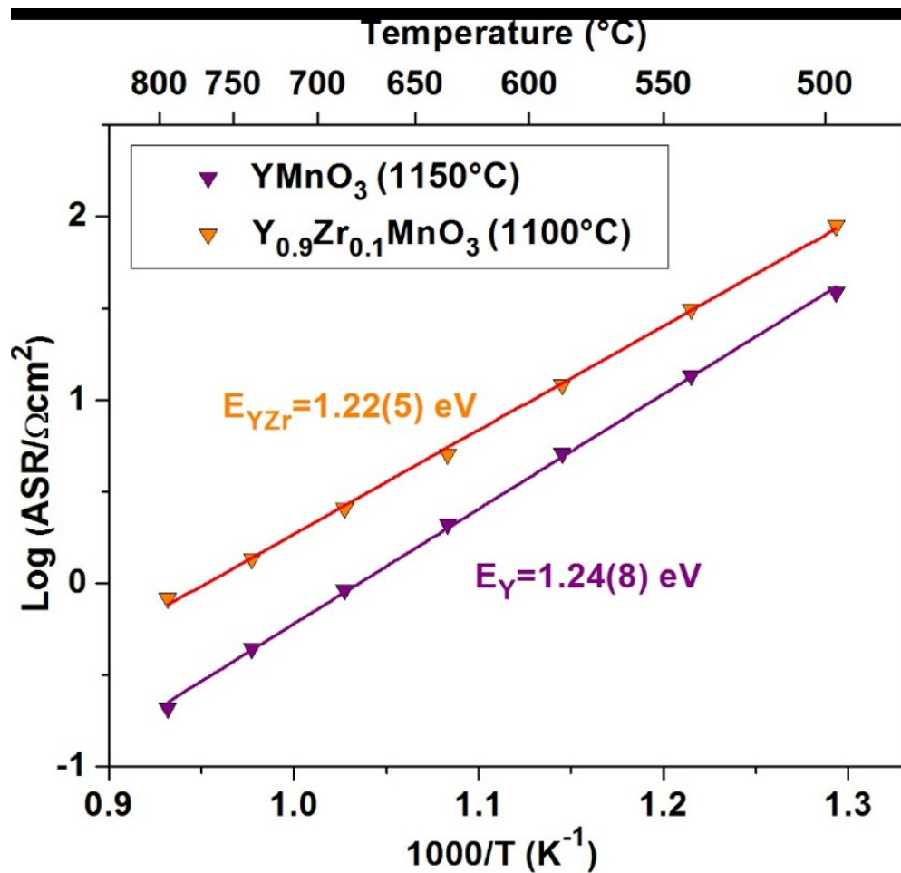
Figure 9. Log ASR values vs temperature for symmetrical cells containing \text{YMnO}_3 and \text{Y}_{0.9}\text{Zr}_{0.1}\text{MnO}_3 compound in its optimal conditions.
