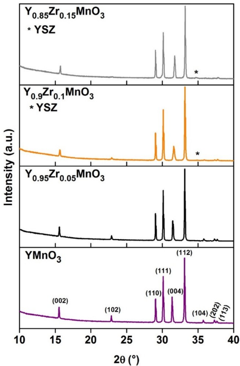
Figure 2. X-Ray diffraction patterns of Y 1-x Zr x MnO 3 (0 ≤ x ≤ 0.15) indexed in P6 3 cm structure. Reproduced with permission from 35.
