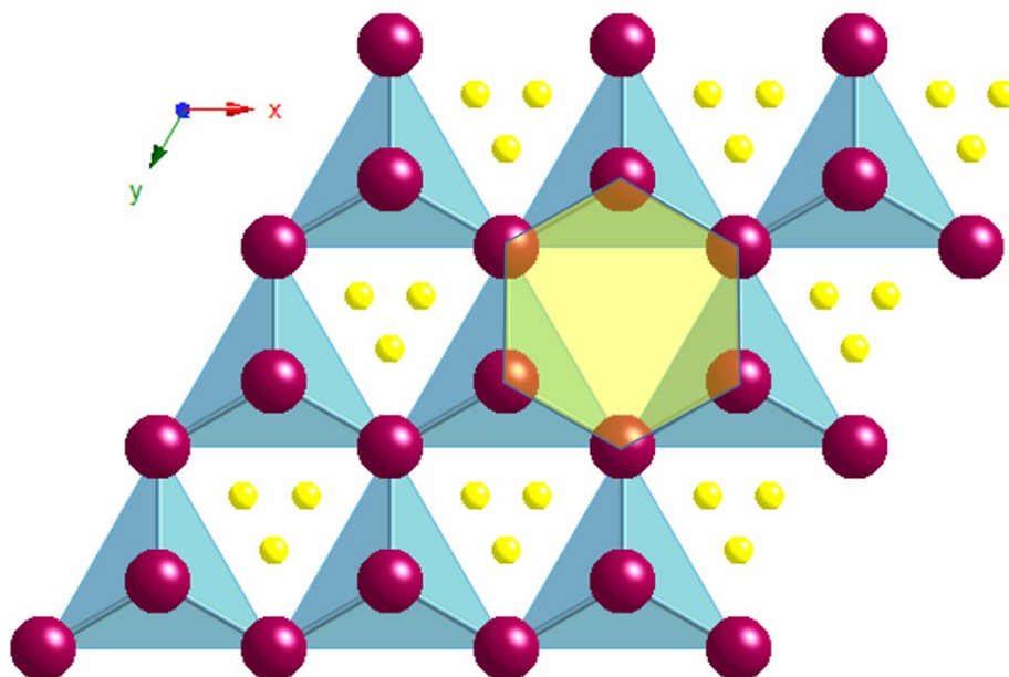
Figure 5. Representation along c axis of P63/mmc Y_{0.9}Zr_{0.1}MnO_{3+\delta} structure evidencing the position of overstoichiometric O3 atoms (in yellow) in the normally empty hexagonal cavities defined by three MnO5 bipyramids. Y atoms have been omitted for clarity.
