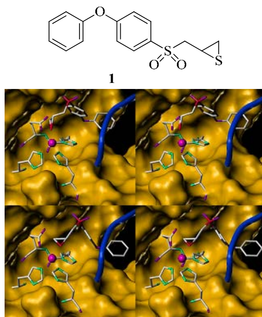
Figure 1. Stereoview representation of compound (R)- 1 (top) and (S)- 1 (bottom)—both enantiomers are equally active against gelatinases—in the active site of MMP-2. The zinc ion is shown as a purple sphere.
