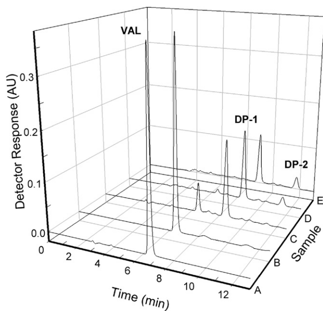
Fig. 2. Chromatograms of VAL and its photodegradation products. (A) Control sample (not exposed). (B) Sample of VAL (1.0 \text{mg ml}^{-1} ) exposed to UV–vis radiation ( \lambda > 320 nm) after the ICH guideline conditions. (C–E) Formation of the degradation products by exposure of a solution of VAL to the metal halide lamp, at different irradiation times (1.5, 3.0 and 4.5 h, respectively).
