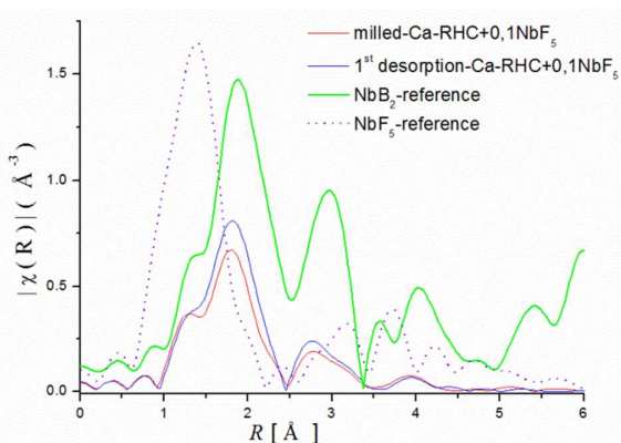
Figure 7. Radial distribution functions (FT-of EXAFS-spectra) of the samples and references.
