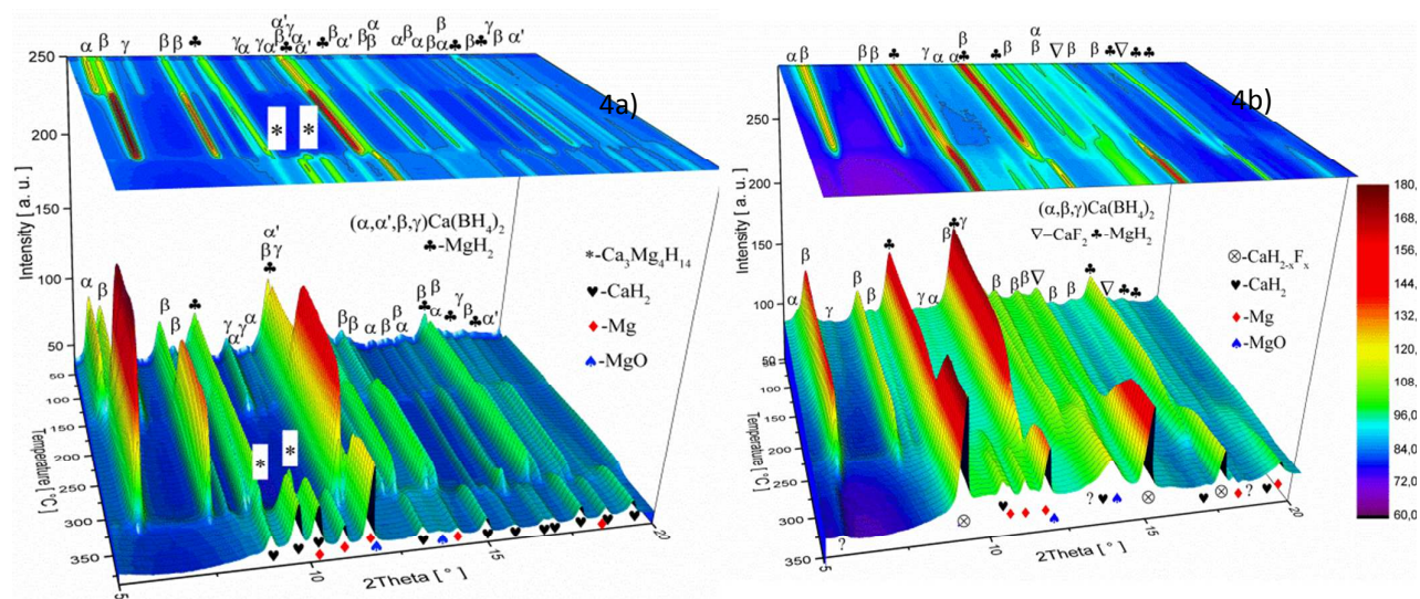
Figure 4. In-situ SR-PXD measurement of Ca-RHC (a) and Ca-RHC+0.1NbF 5 (b) under static vacuum. The samples were heated up from RT up to 400 °C with a heating rate of 3 K/min
