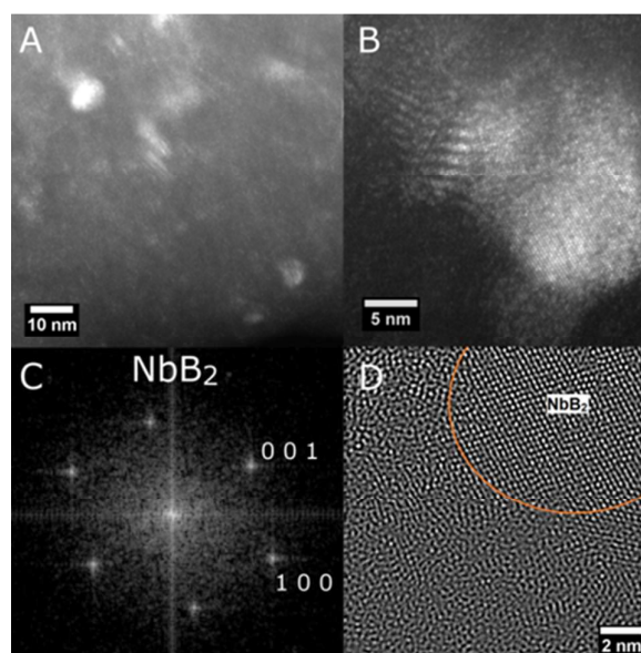
Figure 13. TEM micrographs of Ca-RHC+0.1NbF 5 after the first desorption displaying A) a dark-field where bright regions indicate Nb-rich areas, B) a dark-field of a large Nb-rich region where lattice planes are evident, C) the FFT of a Nb-rich region identifying single crystal NbB 2 , and D) a filtered image demonstrating the amorphous structure surrounding NbB 2 .
