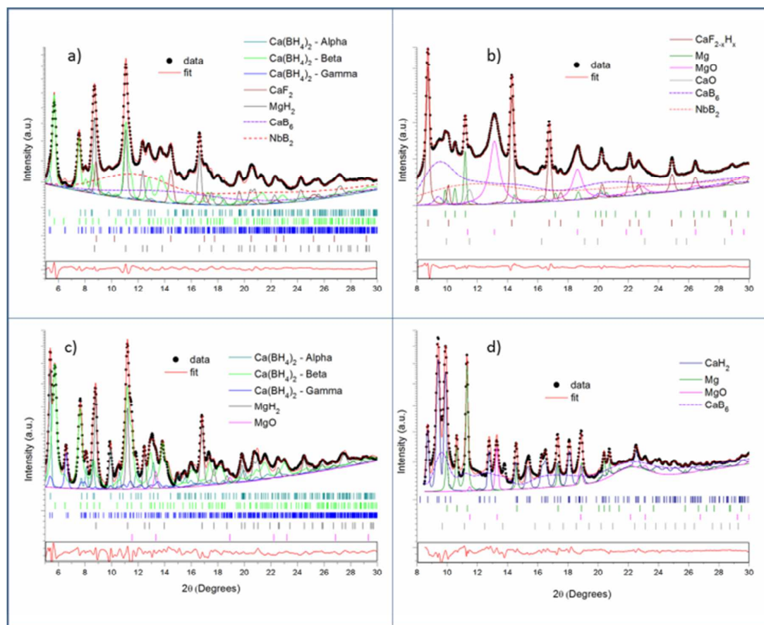
Figure 9. SR-PXD pattern (black dots) collected at room temperature and high temperature respectively for doped - (a), (b), and undoped - (c), (d) - Ca-RHC, and the corresponding simulated profiles. The contribution of each phase with the corresponding Bragg reflections (marked ticks) and the residuals function (red line in the box) are also reported. Only structural models from ICSD database were used.
