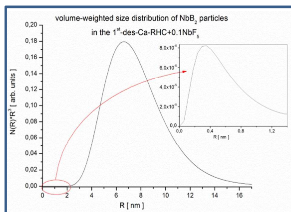
Figure 11. Volume-weighted size distribution of NbB 2 particles in the Ca-RHC+0.1NbF 5 sample after the first desorption.
