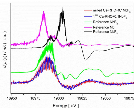
Figure 6. Derivative of XANES structures of the samples and the main references.
