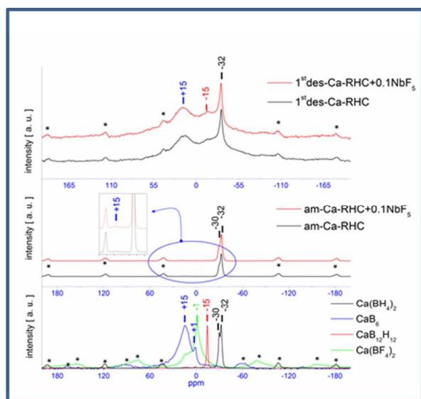
Figure 5. NMR-pattern of once desorbed Ca-RHC/Ca-RHC+0.1NbF 5 (top) and as-milled Ca-RHC/Ca-RHC+0.1NbF 5 (middle) samples with the pattern of references (bottom).
