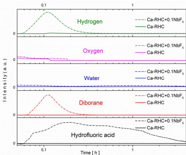
Figure 1. Mass-spectroscopy of the gases released during the milling procedure of pure Ca-RHC and Ca-RHC+0.1NbF 5 .
