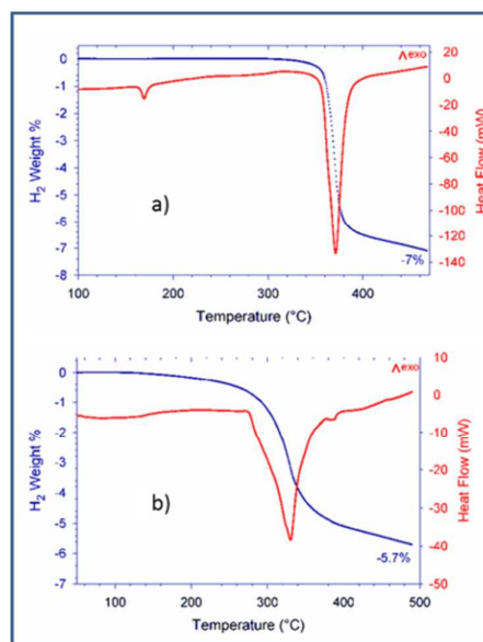
Figure 2. Coupled DSC-manometric curves of Ca-RHC and Ca-RHC+0.1NbF 5 with 3 K/min under vacuum condition.
