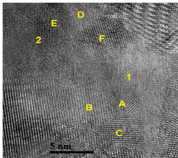
Figure 12. TEM micrograph indicating localised amorphous regions (1) and (2). Attributed phases for the lattice spacing present include: (A) (011) Mg; (B) and (C) (011) CaB 6 ; (D) 1.98 Å (011) hkl reflection CaB 6 (E) and (F) 2.49 Å, Mg.
