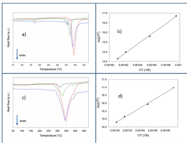
Figure 3. Calorimetric profiles and related Kissinger plot of the undoped (a, b) and the doped (c, d) samples heated from room temperature up to 500 °C at 1 (black line), 3 (green line), 7 (blue line) and 10 (red line) °C/min in vacuum.
