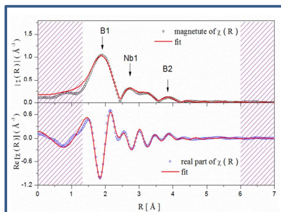
Figure 8. The magnitude (top) and the real part (bottom) of the EXAFS-spectrum of the desorbed \text{Ca-RHC}+0.1\text{NbF}_5 sample in R -space with their corresponding fits.
