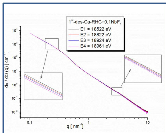
Figure 10. ASAXS curves of Ca-RHC+0.1NbF 5 sample after the first desorption.
