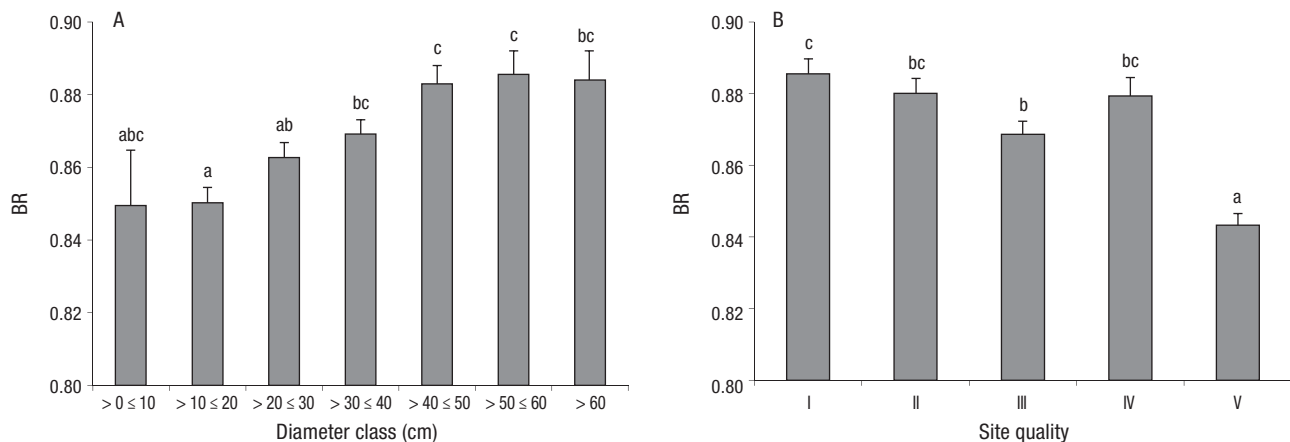
Figure 3. Results of the Analysis of Variance of relationship between volume without and with bark-BR (n = 717) according to: diameter class (A) and site quality (B).
