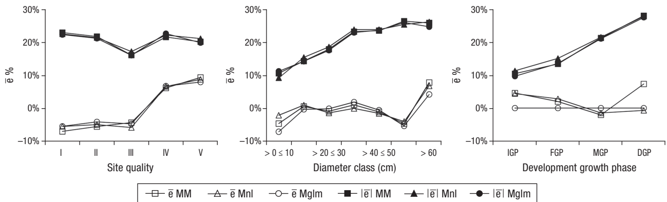
Figure 1. Distribution of the observations according to mean errors ( \% \bar{e} ) and absolute values ( \% |\bar{e}| ). MM: multiple lineal regression model; Mnl: non lineal model; Mglm: generalized linear model, initial growth phase (IGP), final growth phase (FGP), maturing phase (MGP) and decaying phase (DGP).
