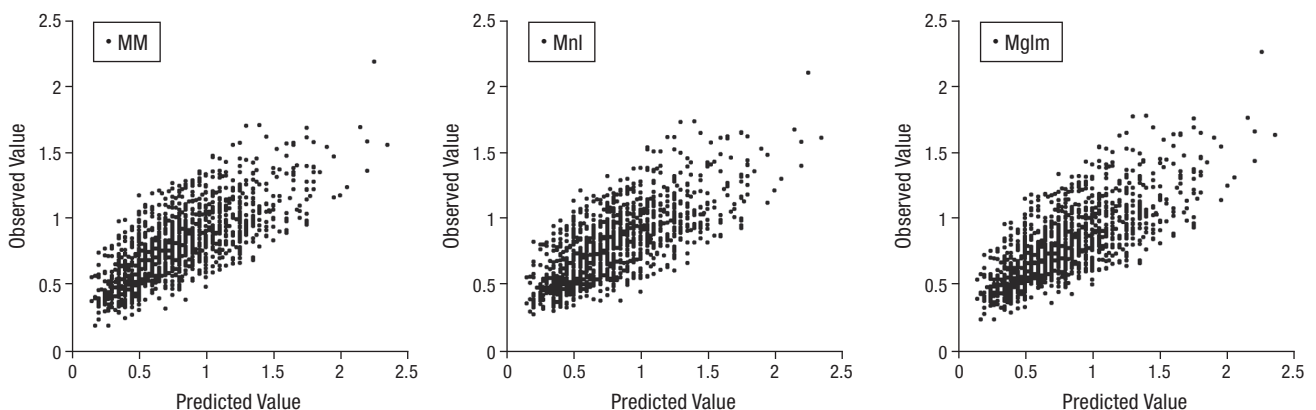
Figure 2. Distribution of the residuals according to observed and predicted values. MM: multiple lineal regression model; Mnl: non lineal model; Mglm: generalized linear model.
