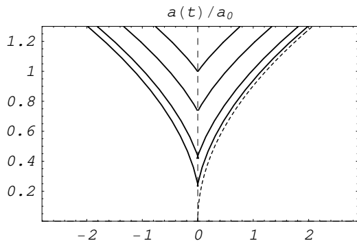
FIG. 1: The scale factor that emerges from Eq. (28), for four different values of the BI constant. From top to bottom in the solid curves: \lambda = 3, 10, 10^2, 10^3 . The dashed curve represents the \omega = 1/3 GR Universe.
