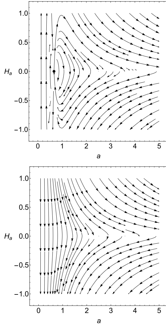
Figure 1. Top panel: phase space of equation (16) when viewed as a system of ODEs in the two variables H_a and a . The parameter \lambda was set as |\lambda| = 9 . The dot represents the critical point a_c . Bottom panel: phase space of equation (16) in the limit |\lambda| \rightarrow \infty which corresponds to standard GR. Note the inversion of the arrows near a = 0 , in contrast to the top panel.
