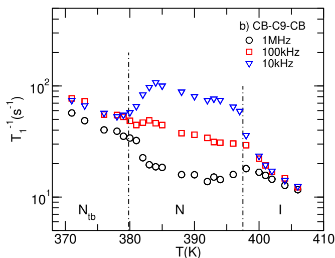
Fig. 9 (Color online) CB-C9-CB experimental spin-lattice relaxation results as a function of the Larmor frequency and temperature. a) T_1^{-1} as a function of the frequency for different temperatures; b) T_1^{-1} as a function of temperature. The dashed lines correspond to the transition temperatures indicated in figure 1.
