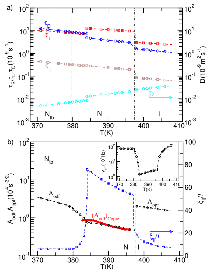
Fig. 14 (Color online) Model fitting parameters as a function of temperature, corresponding to the best fits. In filled red circles are presented the estimated values of A_{\text{ODF}} calculated with the expression for the ODF prefactor of (20) considering distinct elastic constants and viscosities \sqrt{\eta_1/K_1^3 \sum_{m=1}^2 \sqrt{K_1^3 \eta_m / (\eta_1 K_m^2 K_3)}} and the values for the visco-elastic constants reported by Čopić 27 .
