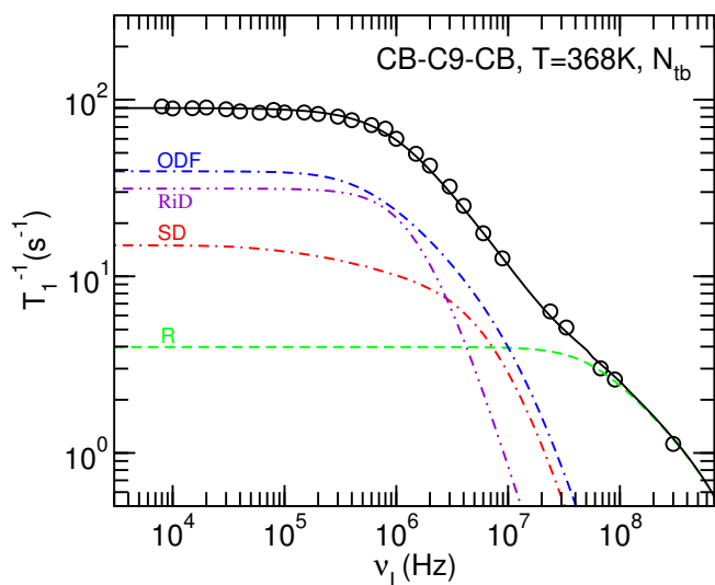
Fig. 15 (Color online) Model fitting of T_1^{-1} dispersion in the N_{tb} phase at T = 368 K, using T_1^{-1} = (T_1^{-1})_R + (T_1^{-1})_{SD} + (T_1^{-1})_{ODF} + (T_1^{-1})_{RiD} with (14), (16), (19), (20), and (23), as explained in the text. The contributions of SD and R are the same as those of 12(a). The ODF contribution changed to compensate the inclusion of RiD contribution.
