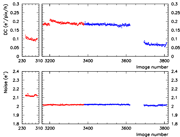
FIG. 13. On-chip noise components in one of the sensors for all exposures considered for this paper. Each point corresponds to a three-hour exposure. The red points are taken during reactor off periods, while the blue ones are during on periods.
