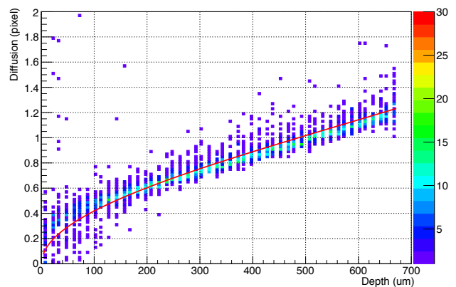
FIG. 9. Two-dimensional histogram illustrating the measurement of the size-depth relationship in one of the sensors. The vertical axis shows the width of the muon segments for each depth in the horizontal axis as measured from muons traversing the CCD. The color scale indicates the number of measurements that lie in each diffusion-depth bin. The solid line is the best fit of Eq. (3) to the distributions.
