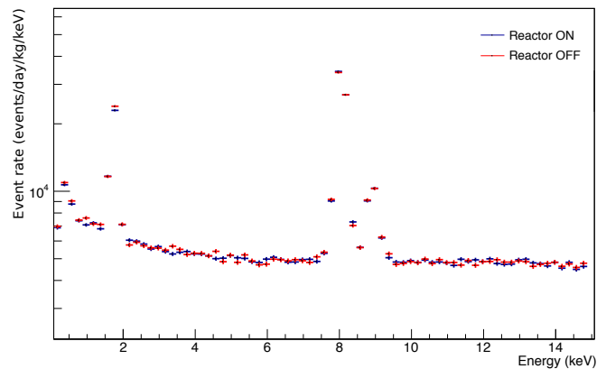
FIG. 18. Energy spectrum for reactor-on and reactor-off data.
