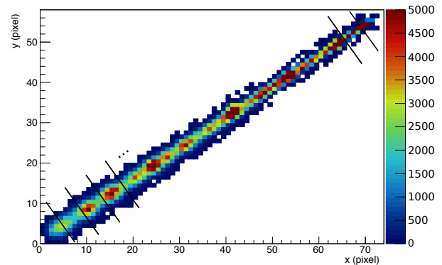
FIG. 8. A typical muon event crossing the entire thickness of the detector where the color scale indicates the charge value of each pixel in arbitrary units. The lines perpendicular to the track define the segments where the transverse standard deviation is measured.
