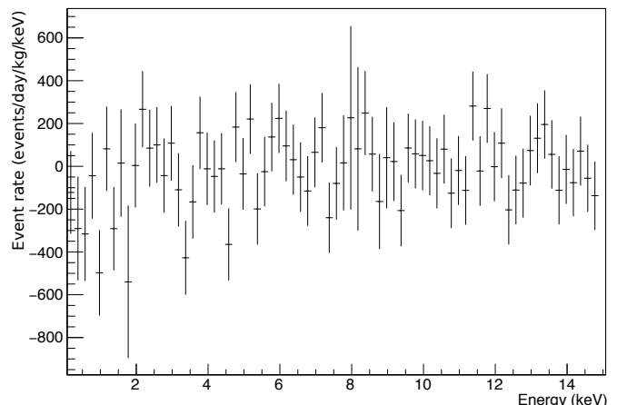
FIG. 19. Energy spectrum difference of reactor-on minus reactor-off data.
