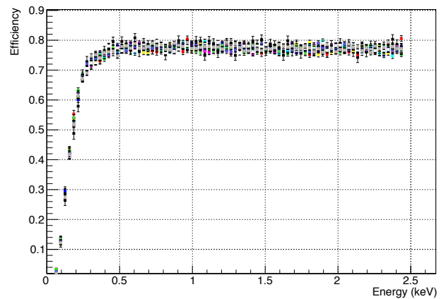
FIG. 15. Reconstructed efficiency of neutrino-like events simulated in the vertical overscan region of one sensor. Each color corresponds to a different sub-run in the detector covering all data used for the analysis in the paper.
