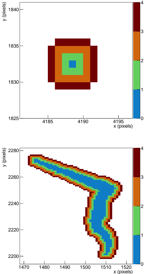
FIG. 5. A cluster with one seed pixel (top) and one with 329 seed pixels (bottom), corresponding to a muon followed by a delta ray. The level of the pixels is given by the color scale on the right.
