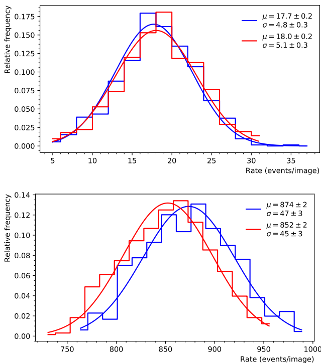
FIG. 12. Unit-normalized histograms of events per image in the energy ranges 3–7 keV (top) and 250–350 keV (bottom), for the reactor on (blue) and off (red) periods. The mean ( \mu ) and width ( \sigma ) of the distributions are also shown.
