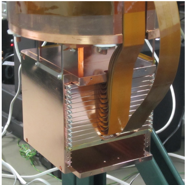
FIG. 2. The cold box with the 14 CCD packages installed. On top is the inner lead shield.
