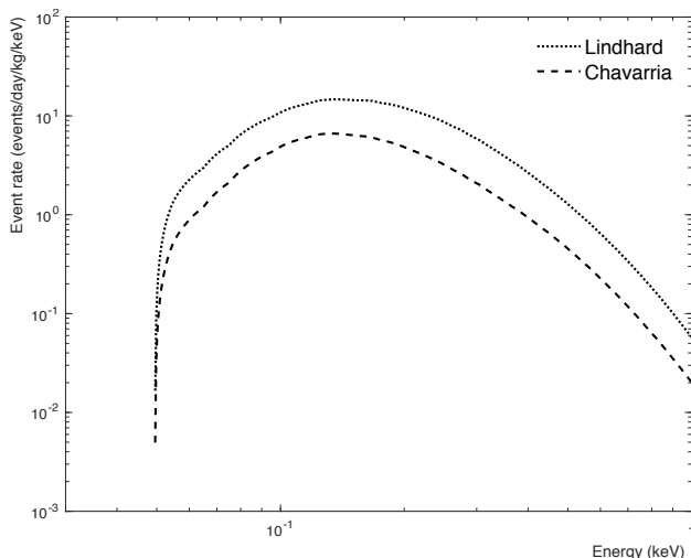
FIG. 17. Observable neutrino recoil spectrum in the CONNIE detector array using two versions of the quenching factor measured from Lindhard et al. [57] (dotted line) and Chavarria et al. [52] (dashed line).
