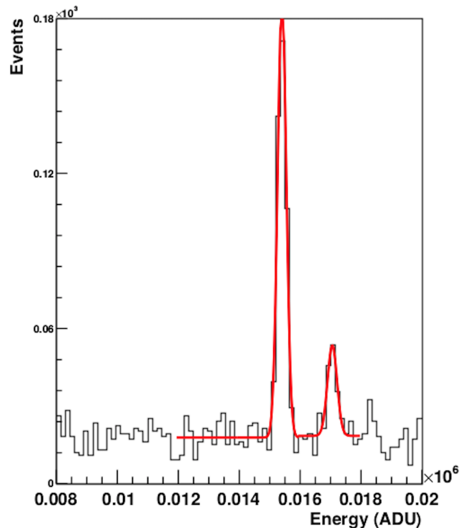
FIG. 6. Energy spectrum (in ADU) around the copper fluorescence peaks for 60 consecutive three-hour exposures. The first peak, corresponding to K\alpha at 8.047 keV, is fitted by a Gaussian and its mean is used to obtain the calibration constant. The second peak is fitted by the same function.
