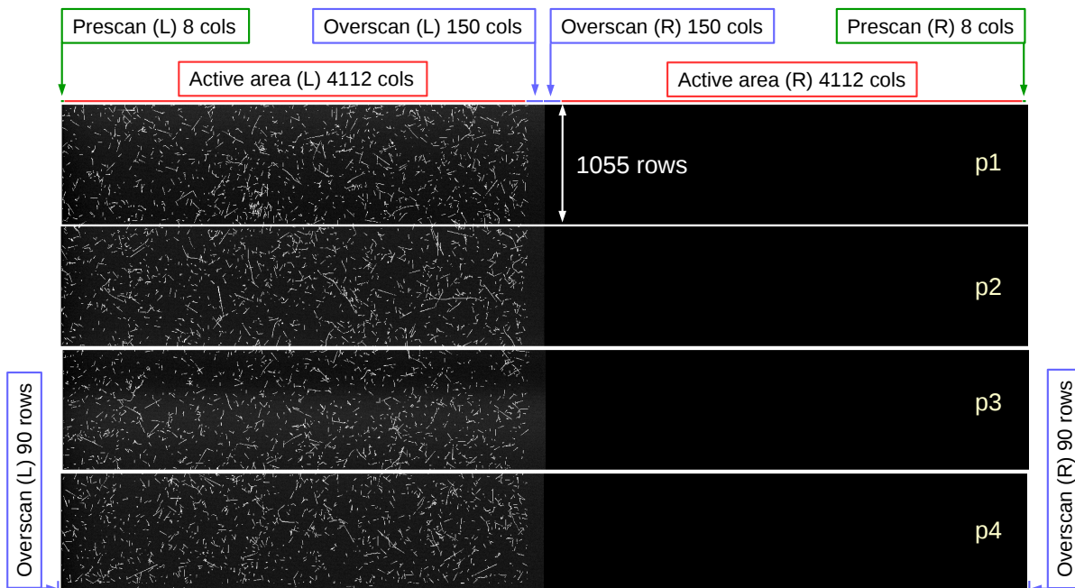
FIG. 4. Schematic representation of a CONNIE image from the standard data acquisition. For memory handling reasons, the images are divided in 4 parts (p1 – p4) as shown here. The charge is moved only to the left (L) amplifier, such that the right one (R) only reads the noise. A few columns with zero exposure time are read prior to moving the charge (prescan) and a larger number is read after the charge has been moved (overscan). After each column is read the readout continues for some more pixels (vertical overscan, thin strip at the bottom of p4).
