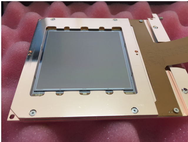
FIG. 1. Image of a package including the CCD, which is glued to a silicon frame, the upper and lower copper frames and the Stage-1 flex cable.
