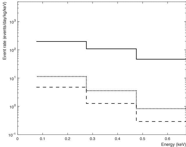
FIG. 20. CE \nu NS event rate: 95% confidence level limit from the reactor on - off measurement (solid line) and neutrino signal expected from the Lindhard [57] (dotted line) and Chavarria [52] (dashed line) quenching factors.
