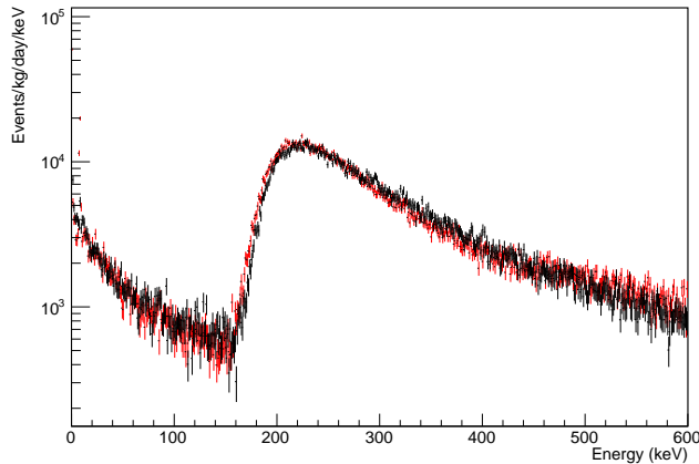
FIG. 10. Comparison of the simulated spectra from muons and data in one of the sensors. The red curve represents data from one of our runs (0.048 kg-day), while the black curve represents the muon contribution obtained with the Geant4 package. The simulated spectrum is based on the expected rate of muons at sea level and has not been fitted to the data.
