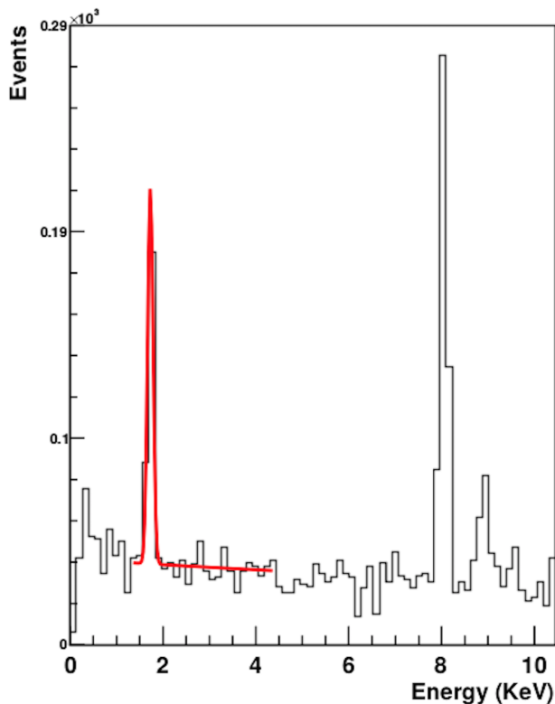
FIG. 7. The calibrated energy spectrum in the region up to 10.5 keV. The Si fluorescence peak at 1.740 keV is fitted by a Gaussian plus an exponential.
