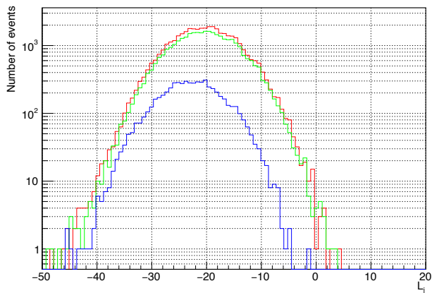
FIG. 14. L_j distribution from simulated noise events for three combinations of DC and RN representative of the selected data.
