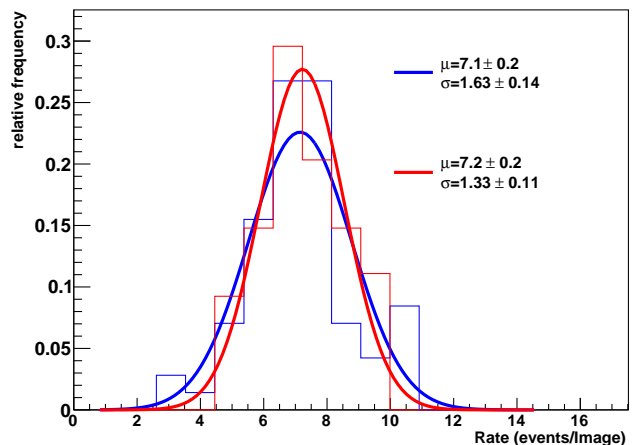
FIG. 11. Top: Unit-normalized distributions of the fitted calibration constant (Cu K\alpha ) from spectra of groups of 5-6 images, for the reactor-on (blue) and reactor-off (red) periods. Bottom: unit-normalized distributions of the event rate under the Cu K\alpha peak calculated as the area of the fitted Gaussian. The mean ( \mu ) and width ( \sigma ) of the distributions are also shown.
