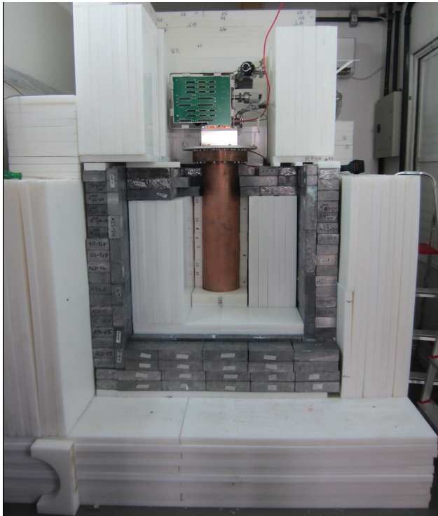
FIG. 3. Image of the CONNIE detector showing the shielding partially disassembled. At the center we see the cylindrical dewar holding the copper box with the CCDs, cables, and inner lead shield. On top of it are the readout electronics. The inner and outer polyethylene layers and the lead layer of the shielding surround the detector.
