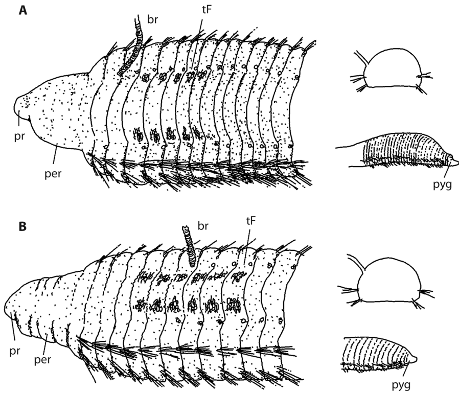
Fig. 3. Schematic drawings of A: Protocirrinera strandloperum sp. nov. and B: P. magalhaesi sp. nov. showing comparatively the diagnostic characters.
