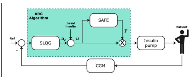
Figure 1. Block diagram of the automatic regulation of glucose algorithm.
