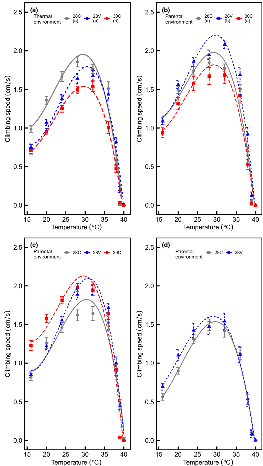
FIGURE 2 Ontogenetic and Transgenerational effects of temperature on thermal performance curve. Offspring and parents were reared in one of three environments 28 \pm 0^\circ\text{C} (28C), 28 \pm 4^\circ\text{C} (28V), and 30 \pm 0^\circ\text{C} (30C). Thermal performance curves were fit to a third-order polynomial function. (a) Ontogeny, climbing speed of flies reared at 28C, 28V, and 30C. (b–d). Transgenerational effects of the thermal environment. The climbing speed of flies reared at 28C, 28V, and 30C respectively. Eggs from flies reared at 30C did not hatch at 30C. Shapes and colors indicate the thermal environment experienced by of parental population. Different letters indicate a significant difference between groups
