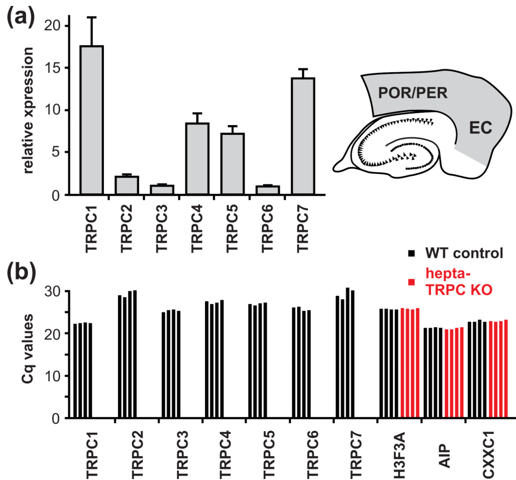
Figure 2. qPCR analysis of the Trpc subunits. (a) qPCR analysis of the Trpc subunits made by RNA isolated from the entorhinal cortex (EC) together with the perirhinal cortex (PER) and the postrhinal cortex (POR). Quantitative expression analysis was performed using high efficiency probe-based assays. Data are given as mean \pm SD (four animals). (b) qPCR analysis using SYBR green I assays specifically designed to verify the respective Trpc deletion in brain tissue of hepta-TRPC KO mice. The primer efficiency varied between assays and accordingly the level of expression is displayed as Cq values. Each bar represents the value of one animal.
