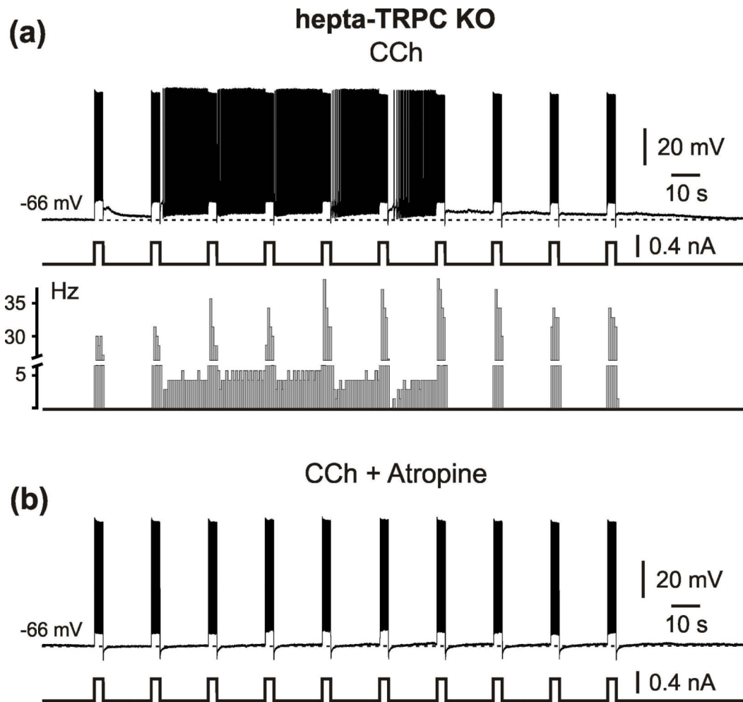
Figure 6. Activity dependent modulation of graded persistent firing in hepta-TRPC knockout mice. (a) Specimen trace showing that repetitive depolarizing current step gives initially increases of stable discharge rate followed, however, by its discrete decreases and full termination. The lower diagram correspond to the peristimulus histograms (bin width 700 ms). (b) Repetitive stimulation in same neuron after adding atropine. Recording was performed in the presence of CCh, CNQX, APV and picrotoxin.
