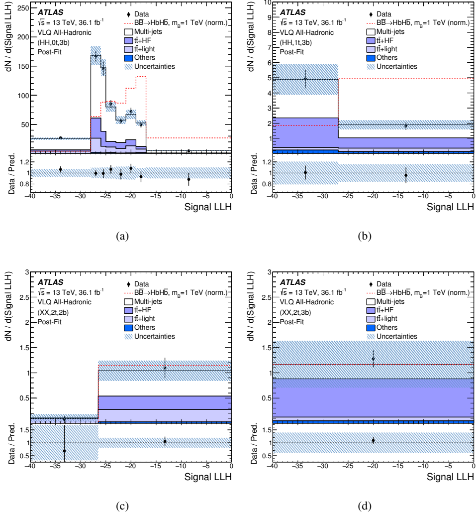
Figure 12: Comparison between data and prediction for the signal LLH distribution after the fit to the data under the background-only hypothesis for the (a) (HH,0t,3b), (b) (HH,1t,3b), (c) (XX,2t,2b) and (d) (XX,2t,3b) signal regions. The contribution labeled ‘Others’ is the combination of single-top-quark and t\bar{t} + X backgrounds. The distributions show the number of events per width of 1.0 in the x -axis. The hatched area represents the total uncertainty of the background. The underflow and overflow are included in the first and last bins, respectively. A hypothetical signal for \mathcal{B}(B \rightarrow Hb) = 100\% and m_B = 1 TeV is shown overlaid, normalized to the integral of the total background.
