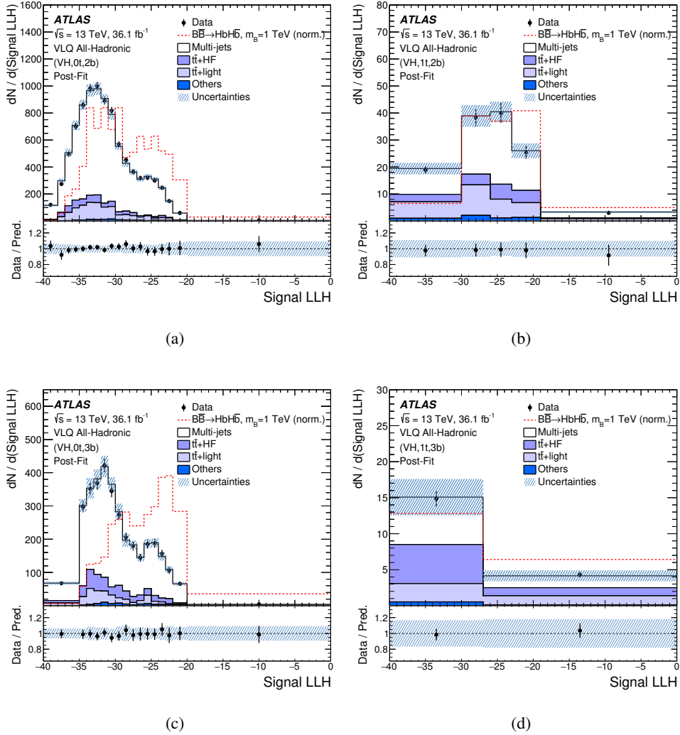
Figure 11: Comparison between data and prediction for the signal LLH distribution after the fit to the data under the background-only hypothesis for the (a) (VH,0t,2b), (b) (VH,1t,2b), (c) (VH,0t,3b) and (d) (VH,1t,3b) signal regions. The contribution labeled ‘Others’ is the combination of single-top-quark and t\bar{t} + X backgrounds. The distributions show the number of events per width of 1.0 in the x -axis. The hatched area represents the total uncertainty of the background. The underflow and overflow are included in the first and last bins, respectively. A hypothetical signal for \mathcal{B}(B \rightarrow Hb) = 100\% and m_B = 1 TeV is shown overlaid, normalized to the integral of the total background.
