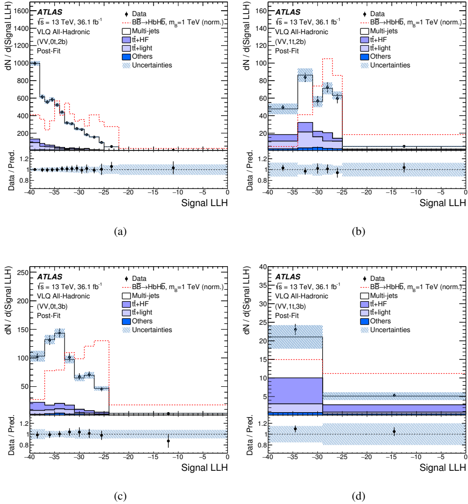
Figure 10: Comparison between data and prediction for the signal LLH distribution after the fit to the data under the background-only hypothesis for the (a) (VV,0t,2b), (b) (VV,1t,2b), (c) (VV,0t,3b) and (d) (VV,1t,3b) signal regions. The contribution labeled ‘Others’ is the combination of single-top-quark and t\bar{t} + X backgrounds. The distributions show the number of events per width of 1.0 in the x -axis. The hatched area represents the total uncertainty of the background. The underflow and overflow are included in the first and last bins, respectively. A hypothetical signal for \mathcal{B}(B \rightarrow Hb) = 100\% and m_B = 1 TeV is shown overlaid, normalized to the integral of the total background.
