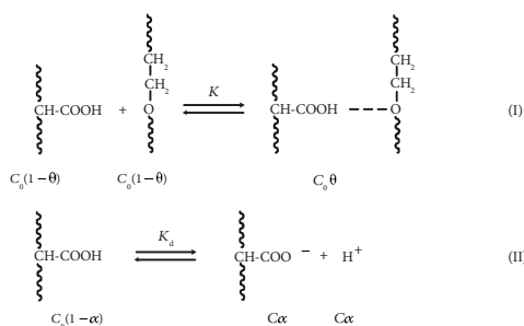
FIGURE 1: Scheme of the equilibrium reactions involved in the complexation reaction between PAA and PEG.
