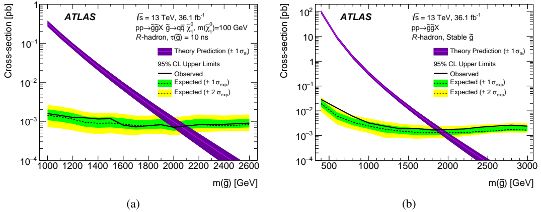
Figure 5: The 95% CL upper limit on the cross-section as a function of mass for (a) gluinos with lifetime \tau = 10 ns decaying into q\bar{q} and a 100 GeV neutralino and for (b) detector-stable gluinos, with the observed limit shown as a solid black line. The predicted production cross-section values are shown in purple along with their uncertainty. The expected upper limit in the case of only background is shown by the dashed black line, with a green \pm 1\sigma and a yellow \pm 2\sigma band. Theory cross-sections are from Refs. [42–46].
