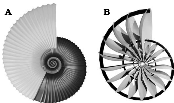
Fig. 7. The final simplified model of the conch of Maorites seymourianus . A. External elements of the conch in lateral view, the smooth areas emulate rectiradiate constrictions; the phragmocone in black, the body chamber in grey. B. Internal elements within the phragmocone; the siphuncle in black, the septa in grey.
