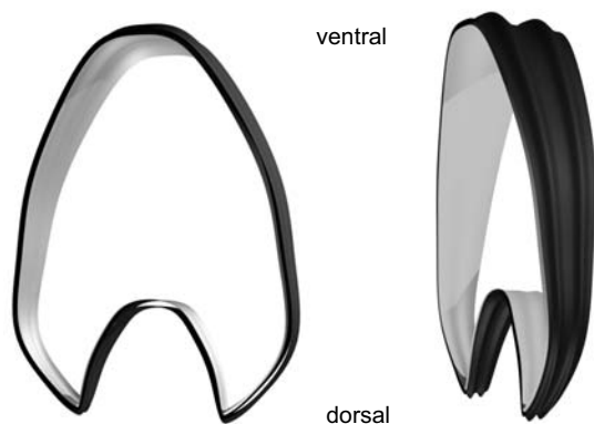
Fig. 5. Final segment in two views showing the rectiradial ribs and the two surfaces emulating the limits of the shell wall. The external layer in black and the internal layer in grey.
