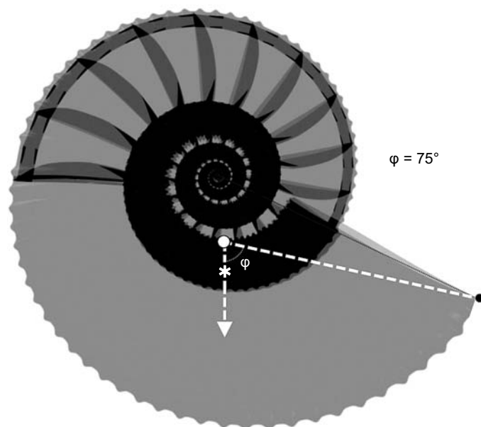
Fig. 10. Model showing the shell orientation ( \phi ) attained during neutral buoyancy for Maorites seymourianus models. White circle, center of buoyancy; asterisk, center of mass.
