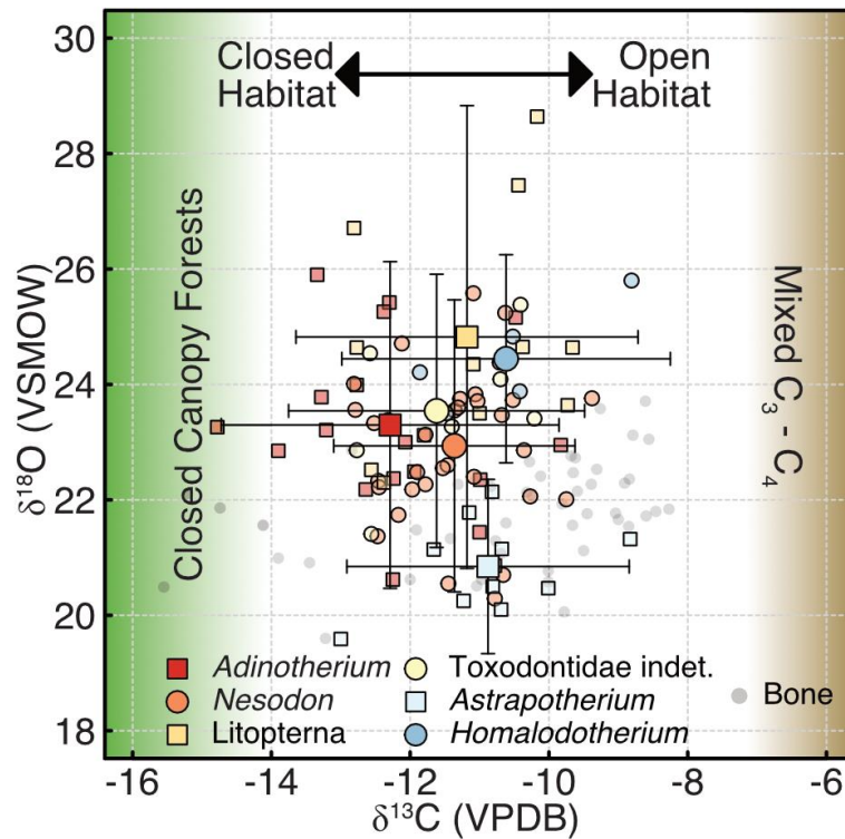
Figure 3. \delta^{13}\text{C} vs \delta^{18}\text{O} values for Santa Cruz Formation herbivores. Large symbols with error bars are the mean \pm 2\sigma for each taxonomic group. Shaded areas at -15‰ and -7.5‰ indicate the transitions for closed canopy forests ( \text{C}_3 ) and mixed \text{C}_3\text{-C}_4 environments (see section 2.2 for details).
