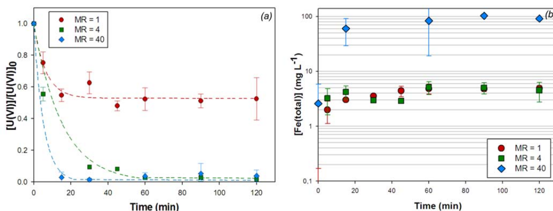
Figure 2: (a) Removal of uranium with nZVI at different Fe:UMRs, [U(VI)] 0 = 0.25 mM, initial pH 5.3, T = 23 ± 1 °C, DO < 0.1 mg L -1 . Dashed curves are only for a better visualization of points and do not correspond to any fitting model; (b) Y-axis semi-log plot for the evolution of [Fe(total)] in each experiment.
