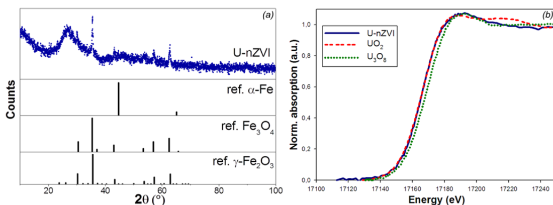
Figure 5: (a) XRD pattern of the solid obtained after removal of U(VI) with nZVI . Spectra of magnetite and maghemite are also shown for comparison. Amorphous signals correspond to the filter used to remove the particles (section 2.4); (b) XANES spectrum of the solid obtained after removal of U(VI) with nZVI . Spectra of UO_2 and U_3O_8 are also shown for comparison.
