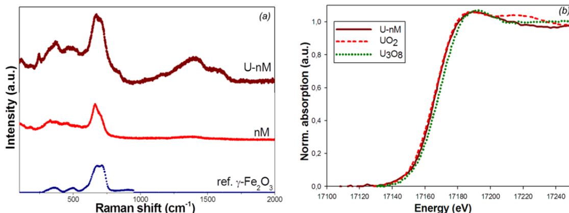
Figure 6: (a) Raman spectra of the solids obtained after U(VI) removal with nM (U-nM), nM before treatment, and maghemite reference; (b) XANES spectrum of the solid obtained after U(VI) removal with nM. Spectra of \text{UO}_2 and \text{U}_3\text{O}_8 are also shown for comparison.
