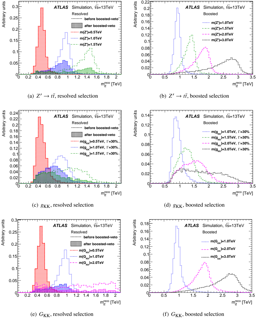
Figure 3: Reconstructed top-quark pairs invariant mass, m_{t\bar{t}}^{\text{reco}} , for simulated signal events satisfying the selection criteria. The Z' in the simulated samples used here has a width of 3% of its mass. The g_{KK} shown here has a width of 30% of its mass and the width of the G_{KK} width varies between 3% to 6% of its mass. The figure shows the distribution including events that may satisfy both the boosted and resolved selections in the line marked as “before boosted-veto”. The line marked as “after boosted-veto” excludes events which satisfy both the boosted and resolved selections from the resolved selection.
