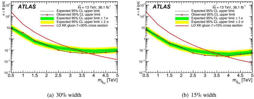
Figure 17: The observed and expected cross-section 95% CL upper limits on the g_{KK} signal for resonance widths of (a) 30% and (b) 15%. The theoretical predictions for the production cross-section times branching ratio of g_{KK} \rightarrow t\bar{t} at the corresponding masses are also shown.
