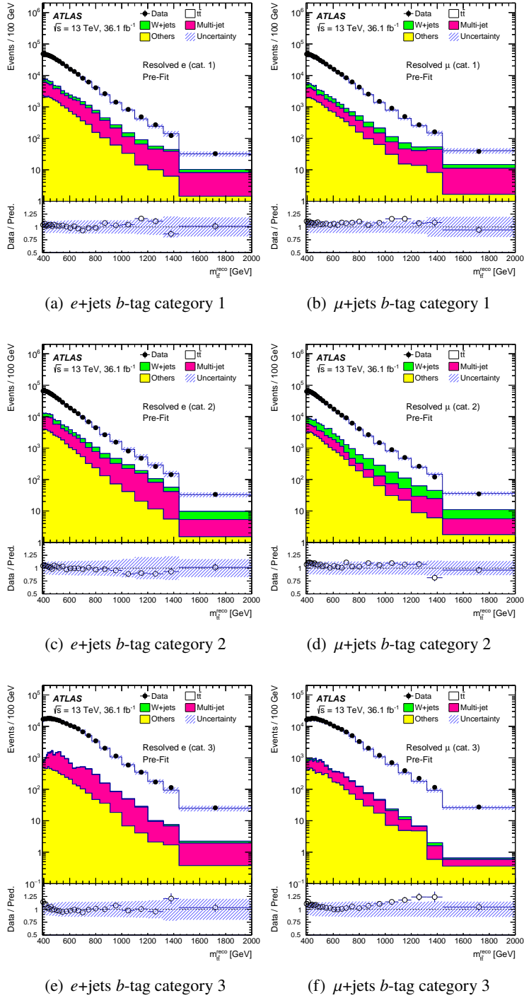
Figure 11: The m_{tt}^{\text{reco}} distribution before the likelihood fit in the resolved selection. The SM background components are shown as stacked histograms. The shaded areas indicate the total systematic uncertainties. The ratio of the data to the total expectation from background processes is shown in the lower panel.
