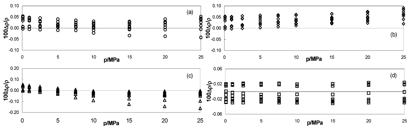
Figure 1. Comparison between the experimental and literature ppT data at different temperatures between 278.15 and 353.15 K for (a) heptane, 27 (b) heptane, 29 (c) heptane, 30 and (d) TEGDME. 28
