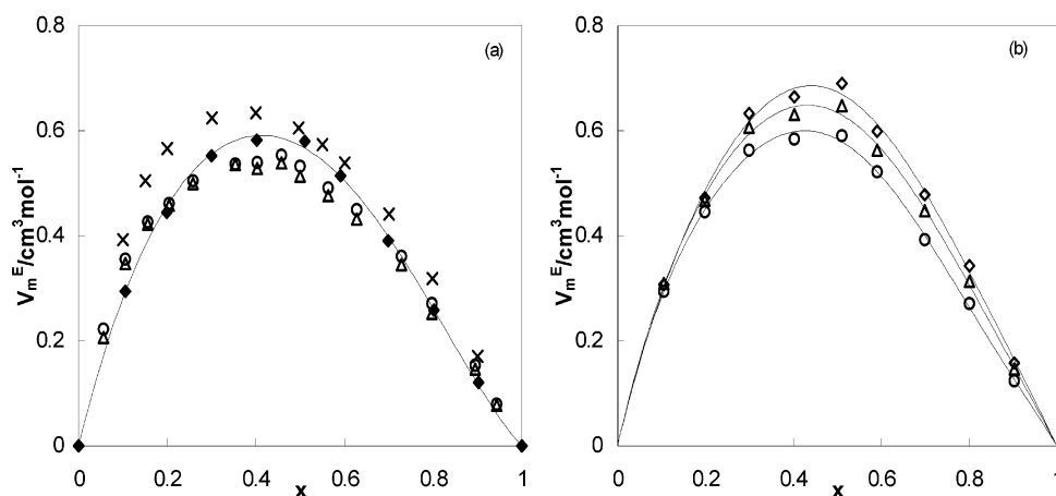
Figure 5. Experimental values of excess molar volumes for (x) TEGDME + (1 - x) heptane versus the mole fraction: (a) at atmospheric pressure for 298.15 K ( \times 19 and \Delta 17 ), 293.15 K ( \blacklozenge , this work), and 288.15 K ( \circ 17 ); (b) at 293.15 K for different pressures ( \circ , 1 MPa; \Delta , 10 MPa; \diamond , 25 MPa).
