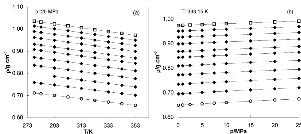
Figure 2. Experimental values of the densities for (x)TEGDME + (1 - x)heptane versus (a) the temperature, T , at 20 MPa and (b) the pressure, p , at 333.15 K: \circ , heptane; \blacklozenge , the following mole fractions of TEGDME (0.10504, 0.19847, 0.29950, 0.40213, 0.50997, 0.59095, 0.69827, 0.80114, and 0.90199); \square , TEGDME.
