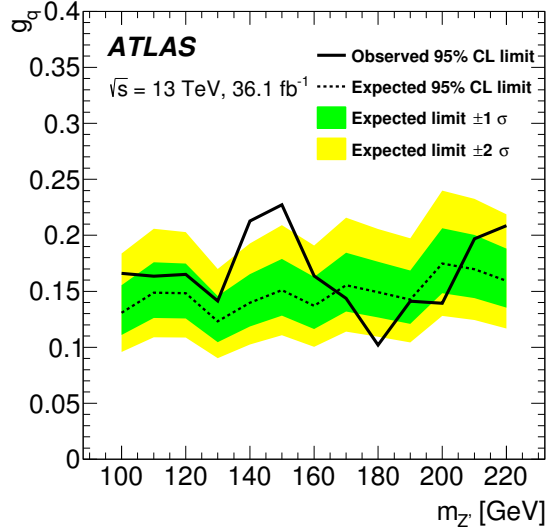
Figure 6: Observed and expected limits at 95% confidence level on the coupling ( g_q ) from the lepto-phobic axial-vector Z' model [30–32], for the combination of the ISR jet and ISR \gamma channels.
