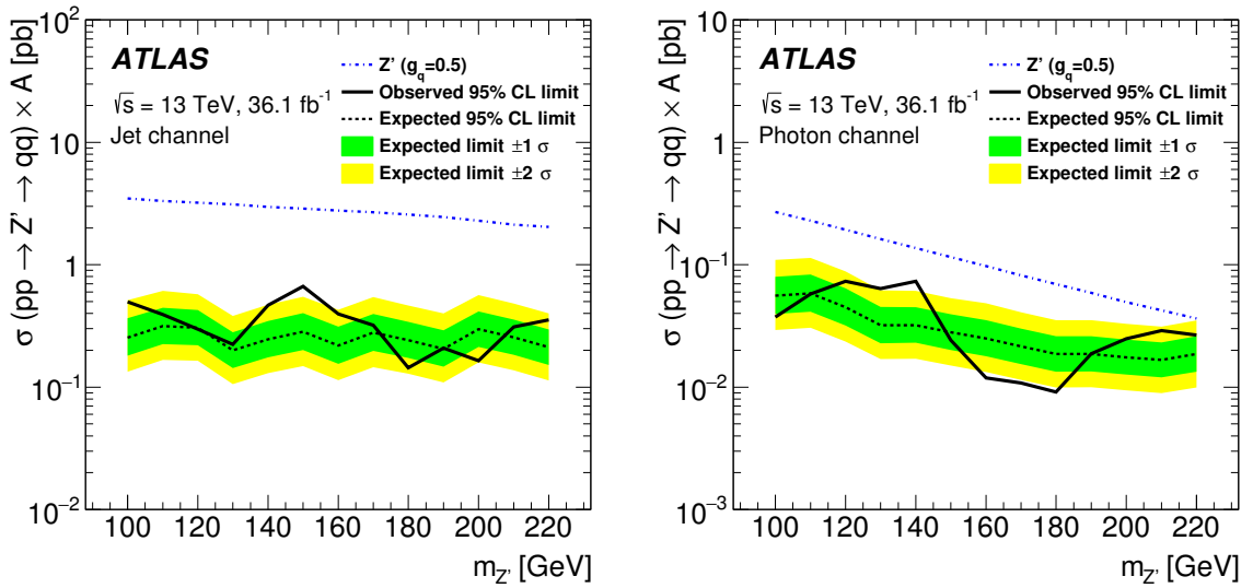
Figure 5: Observed and expected limits at 95% confidence level on the lepto-phobic axial-vector Z' [30–32] production cross section ( \sigma ) times kinematic acceptance ( A , see text for details) in the ISR jet channel (left) and the ISR \gamma channel (right).
