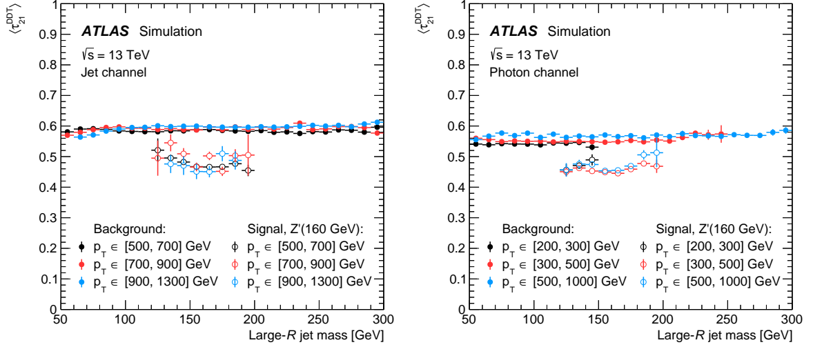
Figure 1: Mean value of \tau_{21}^{\text{DDT}} as a function of the large- R jet mass, for various ranges of large- R jet transverse momentum, for cases where the ISR object is a jet (left) and a photon (right).
