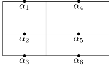
Figure 3: Interpolation points for Q_{12} on S_{ij}
