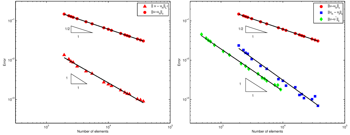
Figure 5: Numerical orders, \varepsilon = 10^{-6} .
