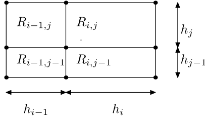
Figure 2: Reference element for the Q_2 -interpolation and region S_{ij}
