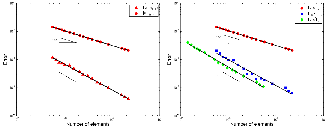
Figure 4: Numerical orders, \varepsilon = 10^{-3} .
