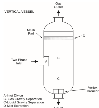
Figure 1. Vertical Phase Separator.
