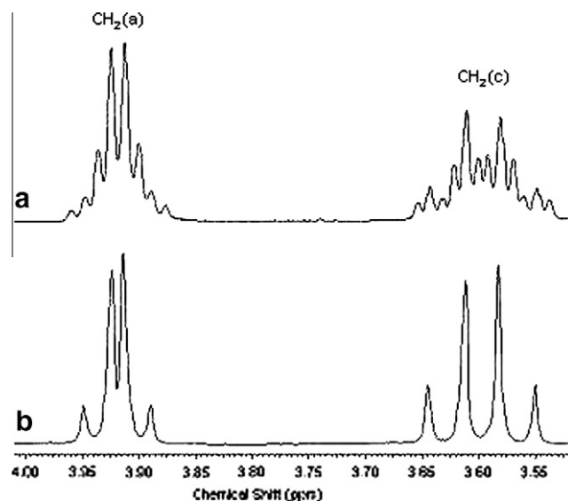
Fig. 5. N -methylene signals of the ^1\text{H} NMR spectrum of compound 1b ( \text{CDCl}_3 ): (a) normal and (b) with simultaneous decoupling of \text{CH}_2(\text{b}) .
