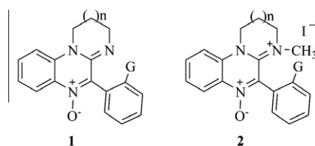
1a, 2a ( n =1, G=CH 3 ); 1b ( n =1, G=Cl); 1c ( n =1, G=Br) 1d, 2b ( n =0, G=CH 3 ); 1e ( n =0, G=Cl)
