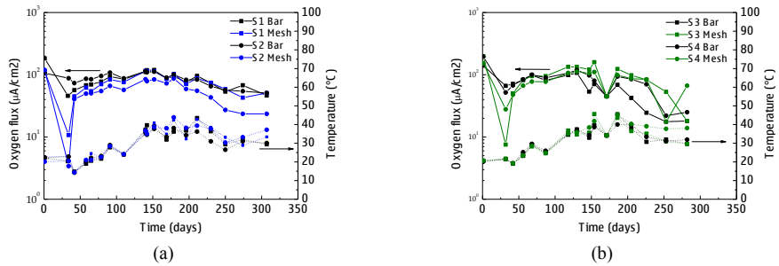
Figure 5. Temporal evolution of the oxygen availability. (a) CPN. (b) CPP.
