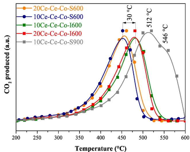
Fig. 5. TPO profiles for diesel soot combustion. A 30 °C-shift shows the enhancement of the catalytic activity achieved when applying the spray deposition method as compared to the drip impregnation method.
