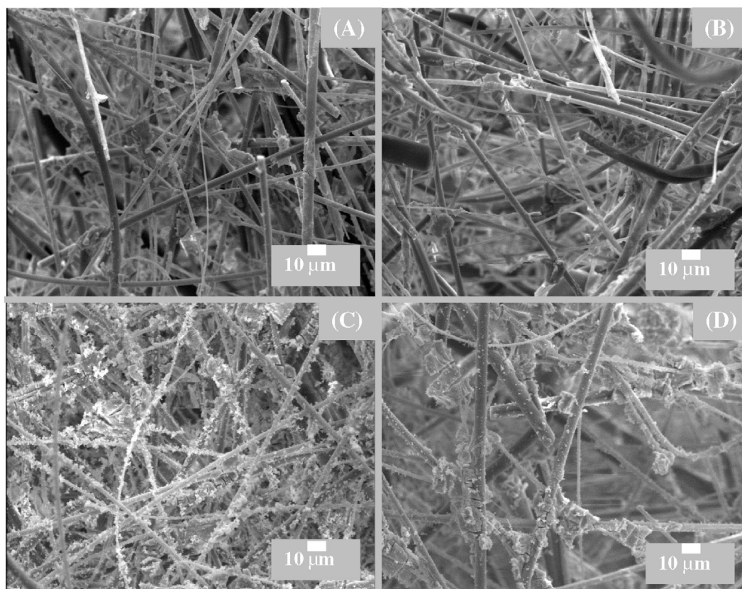
Fig. 2. SEM micrographs. (A) Top face: 10Ce-Ce-Co-600 Imp. (B) Bulk: 10Ce-Ce-Co-600 Imp. (C) Top face: 10Ce-Ce-Co-600 Spray. (D) Bulk: 10Ce-Ce-Co-600 Spray.
