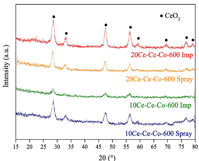
Fig. 4. X-Ray diffraction patterns of the catalytic ceramic papers prepared by the spray deposition (Spray) or the drip impregnation (Imp) methods.
