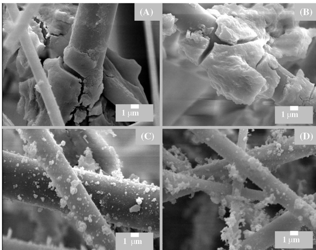
Fig. 3. SEM micrographs. Details of catalytic particles, shapes and sizes obtained after drip impregnation or spray deposition on ceramic papers (A) Top face: 10Ce–Ce–Co–600 Imp. (B) Bulk: 10Ce–Ce–Co–600 Imp. (C) Top face: 10Ce–Ce–Co–600 Spray. (D) Bulk: 10Ce–Ce–Co–600 Spray.
