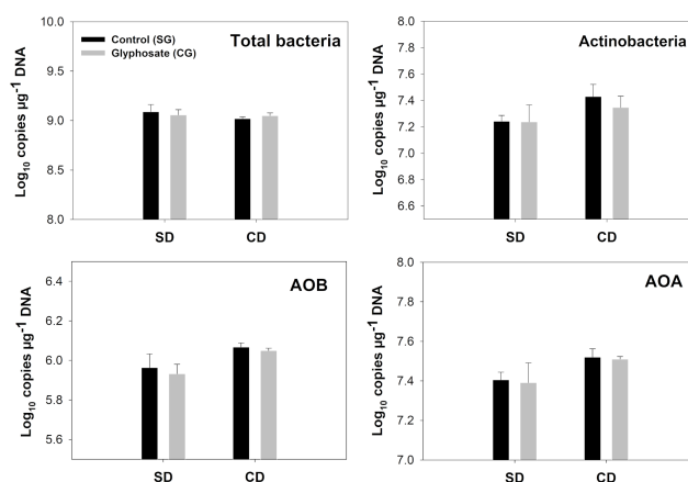
Figure 2. Copy number of indicator genes for total bacteria, Actinobacteria , AOB and AOA. Error bars indicate the standard error of the mean ( n = 3 ). SD/SG: no dry–rewetting disturbance/no herbicide; SD/CG: no dry–rewetting disturbance/herbicide; CD/SG: dry–rewetting disturbance/no herbicide; CD/CG: dry–rewetting disturbance/herbicide.
