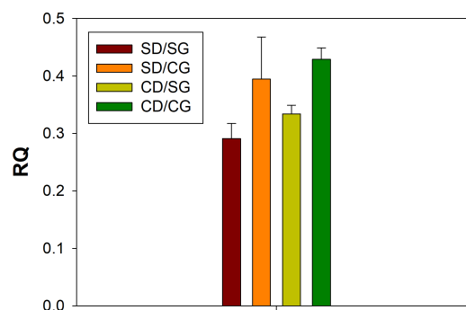
Figure 1. Respiratory quotient (RQ) values. The four treatments are indicated in different colours. Error bars indicate the standard error of the mean ( n = 3 ). SD/SG: no dry–rewetting disturbance/no herbicide; SD/CG: no dry–rewetting disturbance/herbicide; CD/SG: dry–rewetting disturbance/no herbicide; CD/CG: dry–rewetting disturbance/herbicide.
