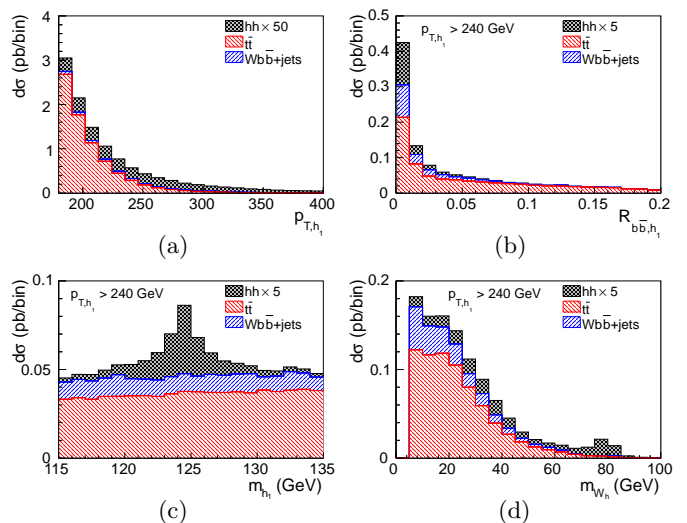
FIG. 2. Distributions for signal and backgrounds of (a) p_{T,h_1} after the basic cuts; and (b) R_{b\bar{b},h_1} ; (c) m_{h_1} , (d) m_{W_h} after the basic cuts and p_{T,h_1} > 240 GeV.
