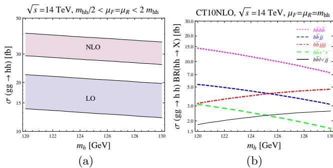
FIG. 1. (a) Scale variation of gluon fusion cross section for Higgs boson pair production, at LO and NLO. (b) cross sections times branching ratios at the 14 TeV LHC, for Higgs boson pair production. We show only the dominant decay modes: bbbb (dots), bbjj (short dashes), bbjjjj (dot-dashes), bb\tau^+\tau^- (long dashes) and bbl\nu jj (solid). Note that the four main decay modes are fully hadronic.
