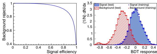
FIG. 3. Outputs of BDT analysis. Left: background rejection vs. signal efficiency. Right: normalized signal and background distributions against BDT response.
