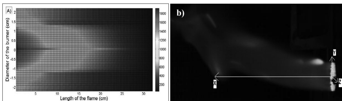
Fig 1 (a) Flame temperature profile; (b) Image of the flame and the axes
