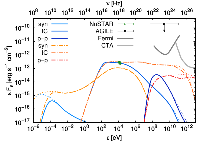
Figure 6. Modelled SED adopting f_{\text{NT},e} = 0.006 , f_{\text{NT},p} = 10 f_{\text{NT},e} , and B_{\text{WCR}} \approx 0.5 G. Solid lines are calculated for an injected particle energy distribution with constant spectral index of p = 3.2 , whereas dash-dotted lines consider a possible hardening of p = 2 in the high-energy spectrum. Dotted lines show the intrinsic emission components before correcting for absorption effects (see Appendix B for details of the model). We also show the NuSTAR data in the 8–18 keV energy range, the AGILE upper-limit assuming a photon index \Gamma = 2 , and the expected sensitivity for 4-yr Fermi -LAT and for 100-h CTA (extracted from Funk et al. 2013).
