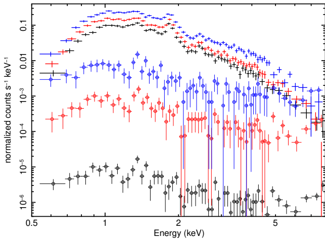
Figure A2. Comparison of the Chandra spectra extracted from a 1'' (black), 10'' (red), and 30'' (blue) region centred at the position of HD 93129A. The crosses represent the source emission and the circles (with errorbars) the background. The spectra are rebinned ( setpl rebin 4 8 in XSPEC) for clarity.
