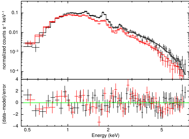
Figure 2. Spectra of HD 93129A as observed with Chandra in 2018 (black) and 2004 (red) extracted from a 1'' circular region. The best-fit model ( [phabs*(vapec_1+vapec_2)] ) is also shown, with the parameters detailed in Table 2.
