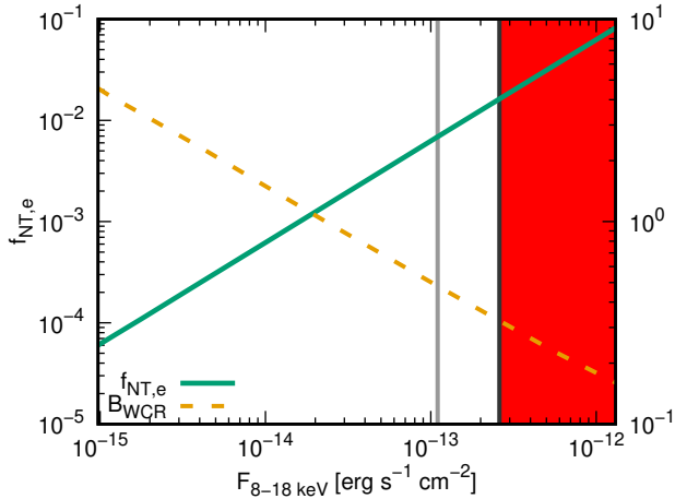
Figure 5. Estimated values of f_{\text{NT},e} and B_{\text{WCR}} in order to obtain a certain X-ray flux in the 8–18 keV. We mark with a dark grey line the strict (most conservative) upper limit for the non-thermal X-ray flux, which assumes that none of the flux observed with NuSTAR comes from HD 93129A. The red region corresponds to values ruled out by the observations. We also show with a grey line the estimated flux value assuming that the relative contribution of HD 93129A to the X-ray flux with respect to the background remains constant above 8 keV (see Sect. 5.1).
