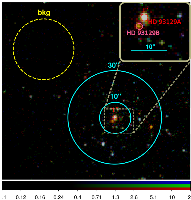
Figure 1. Chandra RGB image from obs. 20152 (red is 0.5–1.2 keV, green is 1.2–2.5 keV, and blue is 2.5–7 keV). Circular regions centred at the position of HD 93129A and of different radii are shown for reference, as well as the selected background extraction region. The position of the source HD 93129B (not part of the system HD 93129A) is also marked for clarity.
