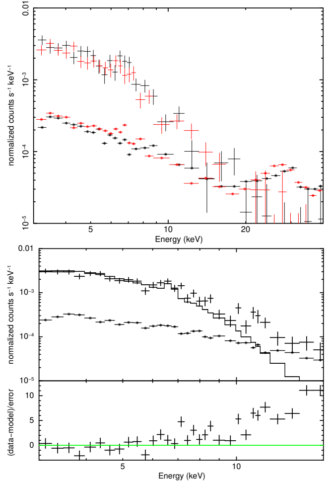
Figure 3. Top: NuSTAR source and background spectra for each observation (first observation is black, second one is red) in the 3–40 keV energy range. The cameras at each observation epoch were co-added with addspec , grouped with ftgroup and rebinned in XSPEC with rebin=4 . Bottom: NuSTAR source and background spectra obtained by co-adding both observations, shown in the 3–20 keV energy range. The model overlaid is the one that fits the Chandra spectrum in the 3–7.5 keV range, with the residuals shown in the bottom panel. The model under-predicts the emission above 8 keV, which can be explained by the presence of either a hotter component or a non-thermal component.
