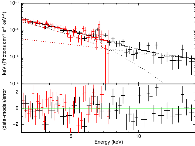
Figure 4. Chandra (red) and NuSTAR (black) spectra for 2018. The fitted model is a [ apec + power-law ], with kT \approx 2.1 keV and \Gamma \approx 1.9 (see text for details).
