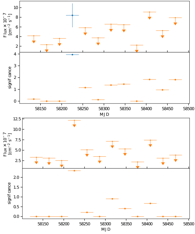
Figure A4. AGILE light-curve in the 50 MeV–100 GeV energy range during 2018. The top panel does not consider emission from \eta -Car, while the bottom panel considers it as an extra background source.
