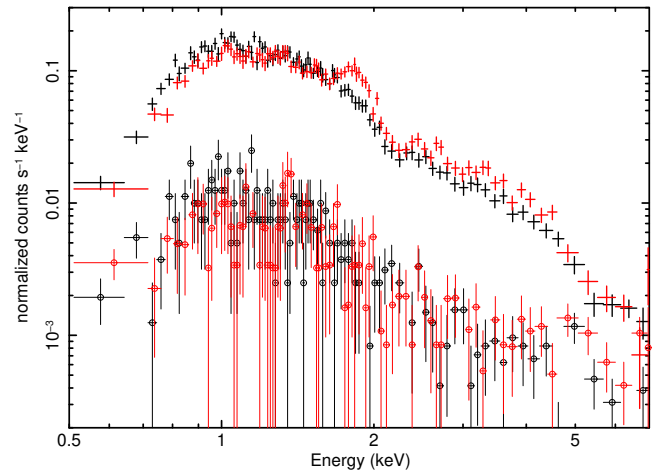
Figure A3. Comparison of the Chandra spectra of the sources within an annulus of outer radius 30'' and inner radius 1'' centred at the position of HD 93129A; black is 2004 and red 2018. The crosses represent the source emission and the circles the background.
