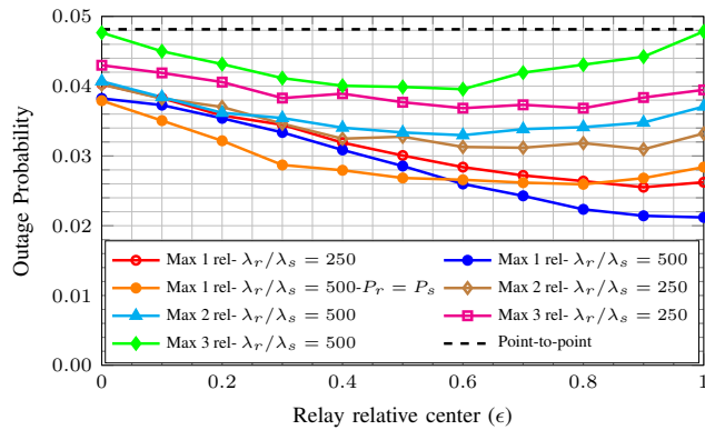
FIGURE 10. Outage probability for MNNC as a function point around which the relays are chosen, one the line between source and destination, for different relative densities. P_r/P_s = -10\text{dB} , \lambda_s = 10^{-4} , R = 1\text{b/use} , \alpha = 4 . OP is optimized w.r.t. the noise compression variance.
