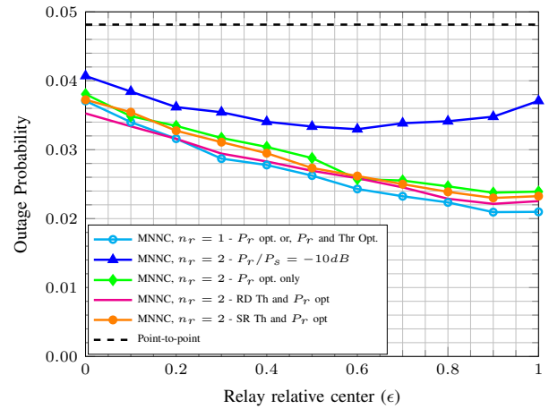
FIGURE 11. Outage probability for MNNC with optimized relay power and thresholds. \lambda_r/\lambda_s = 500 , \lambda_s = 10^{-4} , R = 1\text{b/use} , \alpha = 4 .
