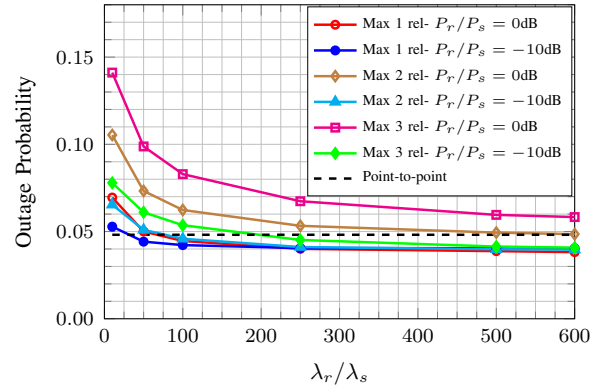
FIGURE 2. Outage probability for ODF as a function of the relative density between relays and sources, for different relay-source relative transmission powers. \lambda_s = 10^{-4} , R = 1 bit/use, \alpha = 4 . Relays are chosen centered around the source ( \varepsilon = 0 ).
