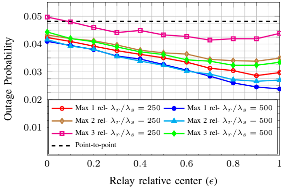
FIGURE 9. Outage probability for NNC as a function point around which the relays are chosen, one the line between source and destination, for different relative densities. P_r/P_s = -10\text{dB} , \lambda_s = 10^{-4} , R = 1\text{b/use} , \alpha = 4 . d = 10 . OP is optimized w.r.t. the noise compression variance.
