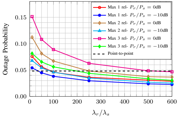
FIGURE 3. Outage probability for NNC as a function of the relative density between relays and sources, for different relay-source relative transmission powers. \lambda_s = 10^{-4} , R = 1\text{b/use} , \alpha = 4 . Relays are chosen centered around the destination ( \epsilon = 1 ). OP is optimized w.r.t. the noise compression variance.
