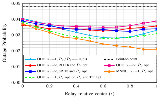
FIGURE 13. Outage probability for ODF with optimized relay power and thresholds, compared to the best performance obtained with MNNC. \lambda_r/\lambda_s = 500 , \lambda_s = 10^{-4} , R = 1\text{b/use} , \alpha = 4 .
