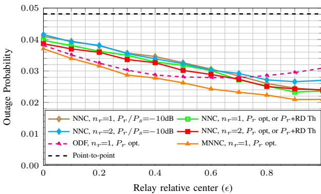
FIGURE 14. Outage probability for NNC with optimized relay power and thresholds, compared to the best performance obtained with MNNC and ODF. \lambda_r/\lambda_s = 500 , \lambda_s = 10^{-4} , R = 1\text{b/use} , \alpha = 4 . OP is optimized w.r.t. the noise compression variance.
