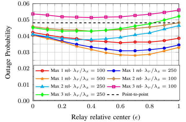
FIGURE 8. Outage probability for ODF as a function point around which the relays are chosen, one the line between source and destination, for different relative densities. P_r/P_s = -10\text{dB} , \lambda_s = 10^{-4} , R = 1\text{b/use} , \alpha = 4 .
