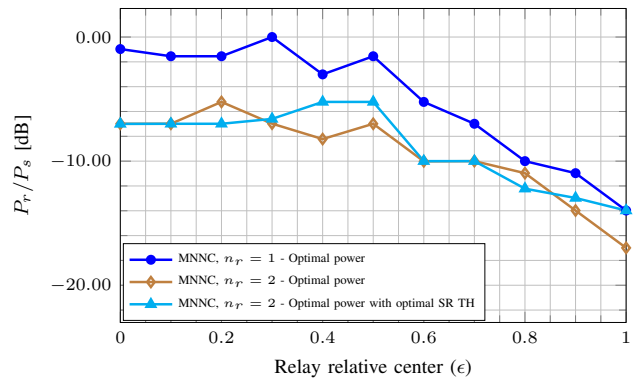
FIGURE 12. Optimal power for MNNC corresponding to the OP of Fig. 11. Using more than one relay allows the reduction of the relay power. \lambda_r/\lambda_s = 500 , \lambda_s = 10^{-4} , R = 1\text{b/use} , \alpha = 4 .
