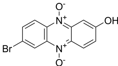
Fig. 1. Molecular structure of 7-bromo-2-hydroxy-phenazine N^5, N^{10} -dioxide (Phenazine).
