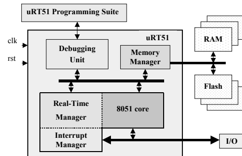
Figure 1. uRT51's architecture layout.
