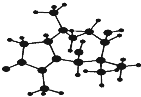
Figure 2. Minimum energy conformation of 1.
