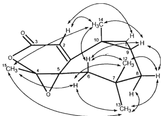
Figure 4. Partial NOEs observed for compound 7.
