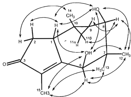
Figure 1. Partial NOEs observed for compound 1.
